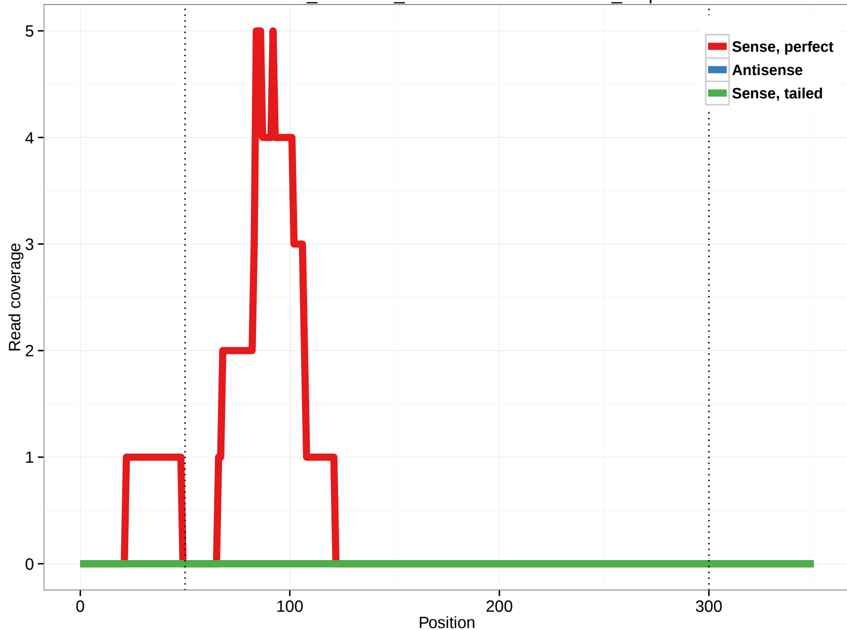
ornAna1_ensGene_ENSOANT00000004998_1.5p
