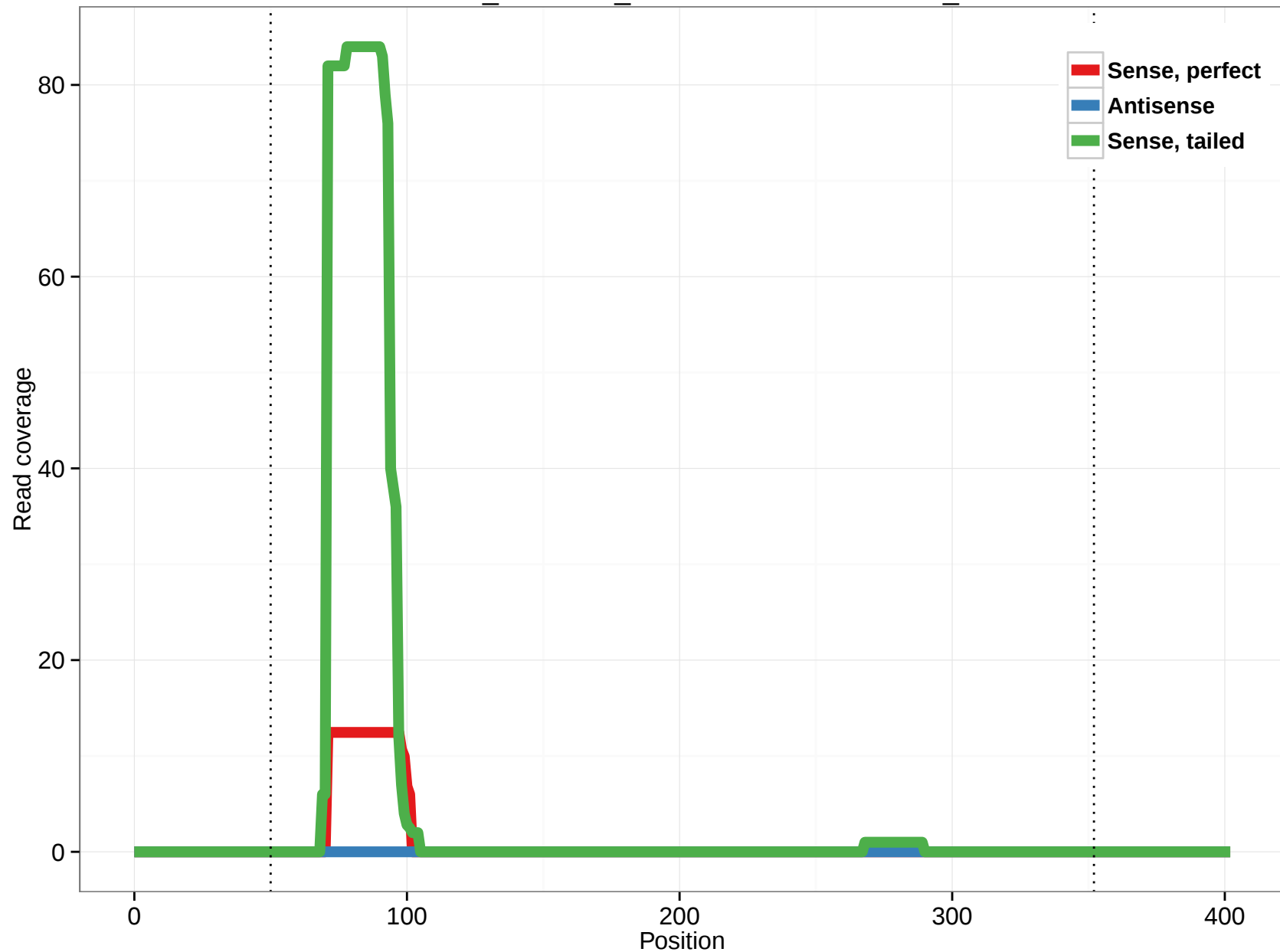
ornAna1_ensGene_ENSOANT00000004930_10
