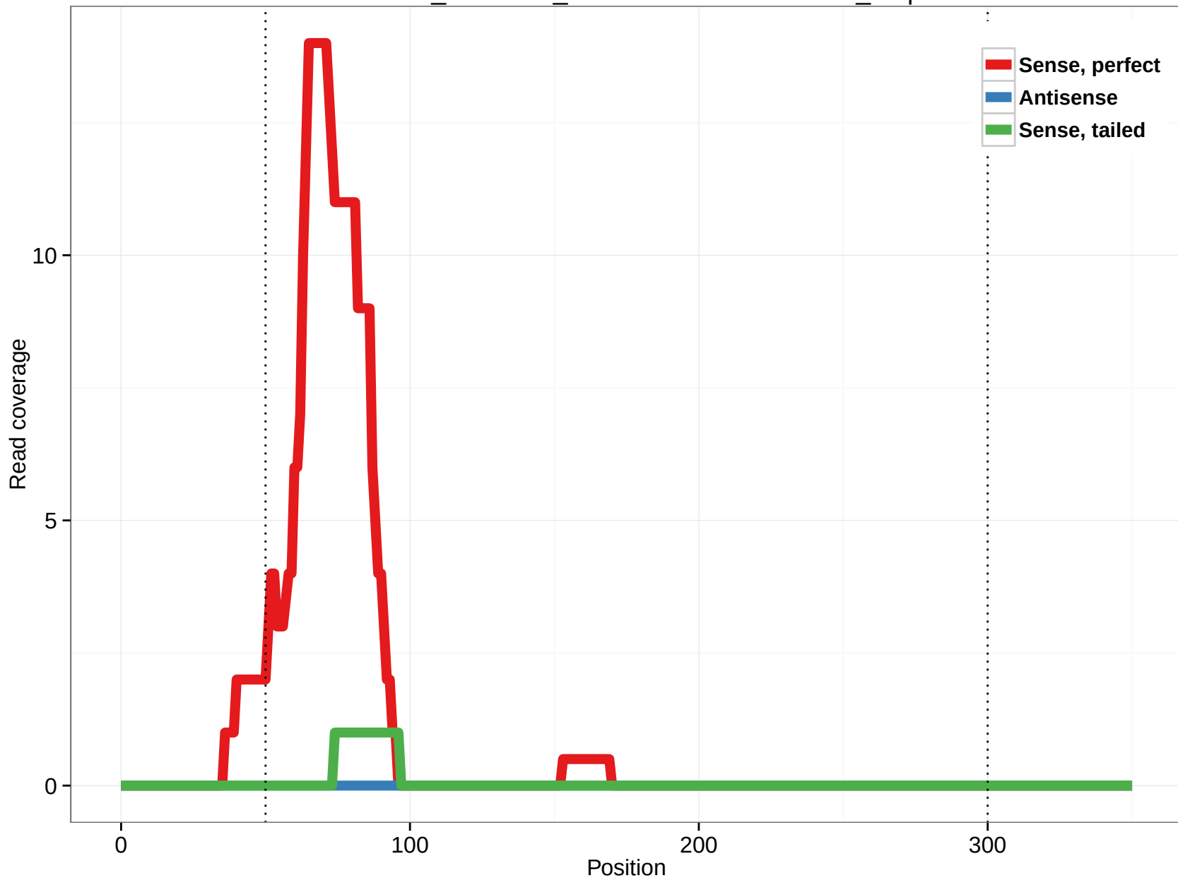
ornAna1_ensGene_ENSOANT00000004927_0.5p
