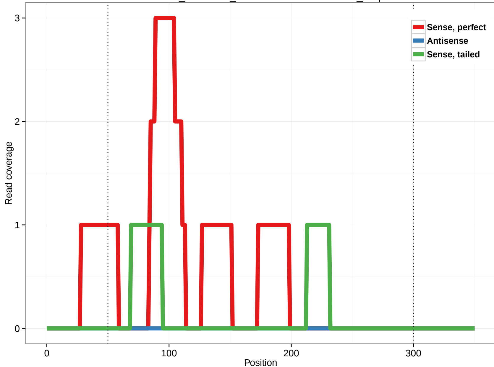
ornAna1_ensGene_ENSOANT00000004906_1.3p
