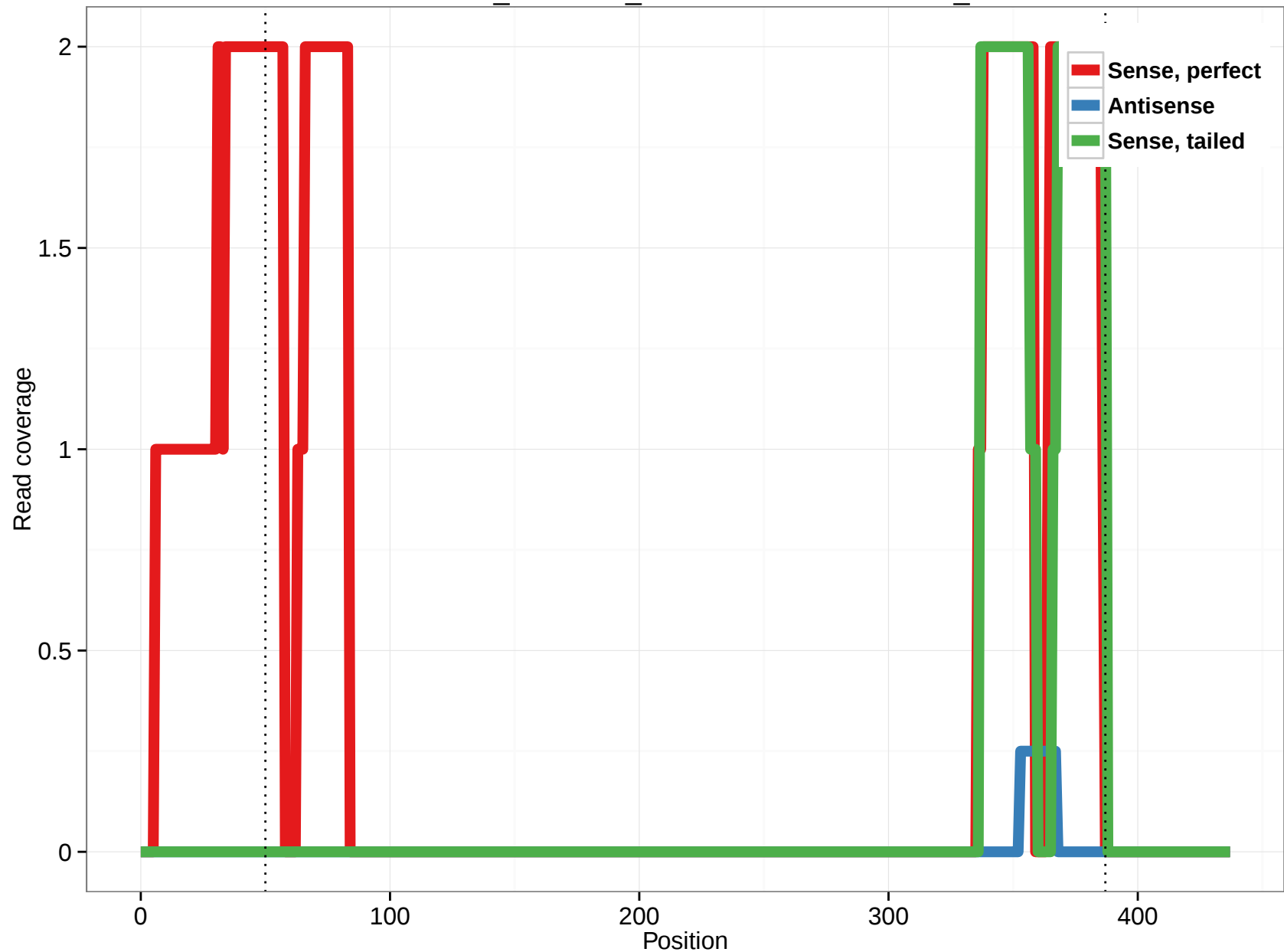
ornAna1_ensGene_ENSOANT00000004846_3
