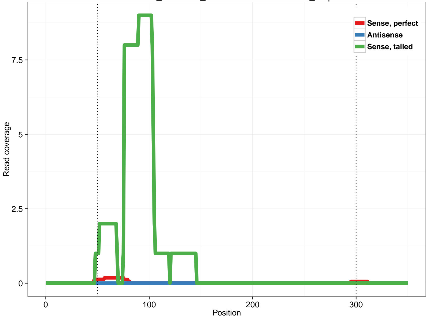
ornAna1_ensGene_ENSOANT00000004813_1.3p
