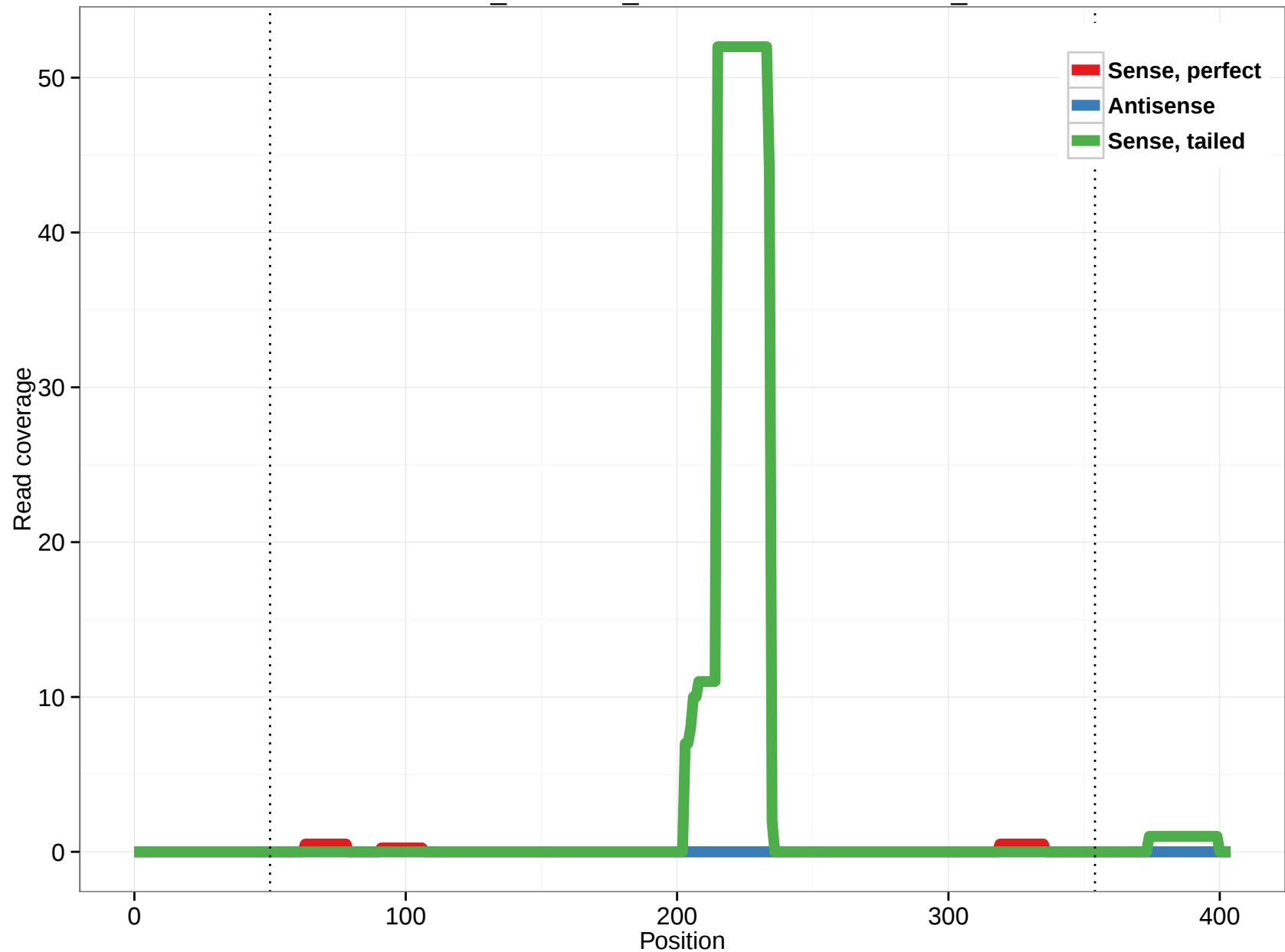
ornAna1_ensGene_ENSOANT00000004734_5
