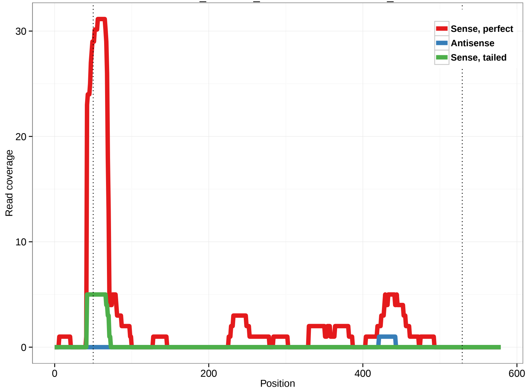
ornAna1_ensGene_ENSOANT00000004698_7
