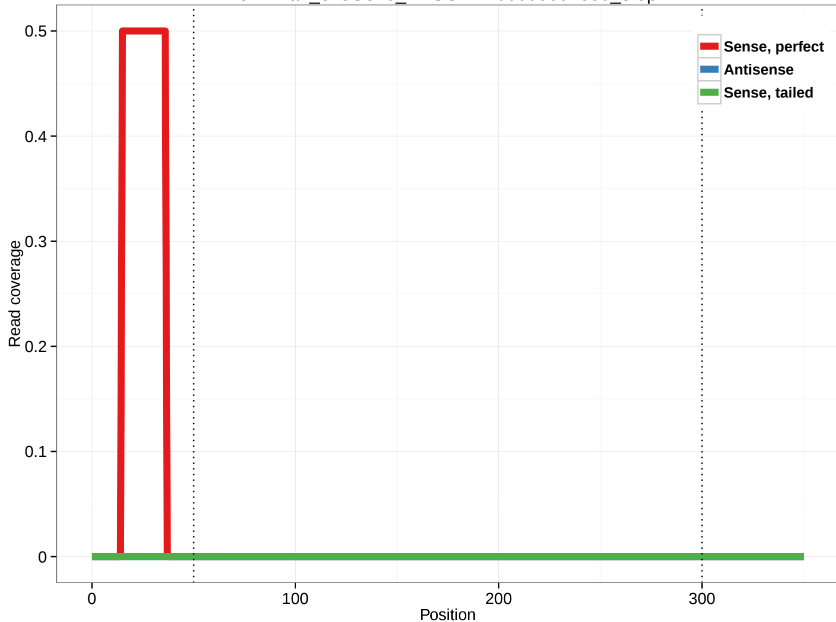
ornAna1_ensGene_ENSOANT00000004680_3.5p
