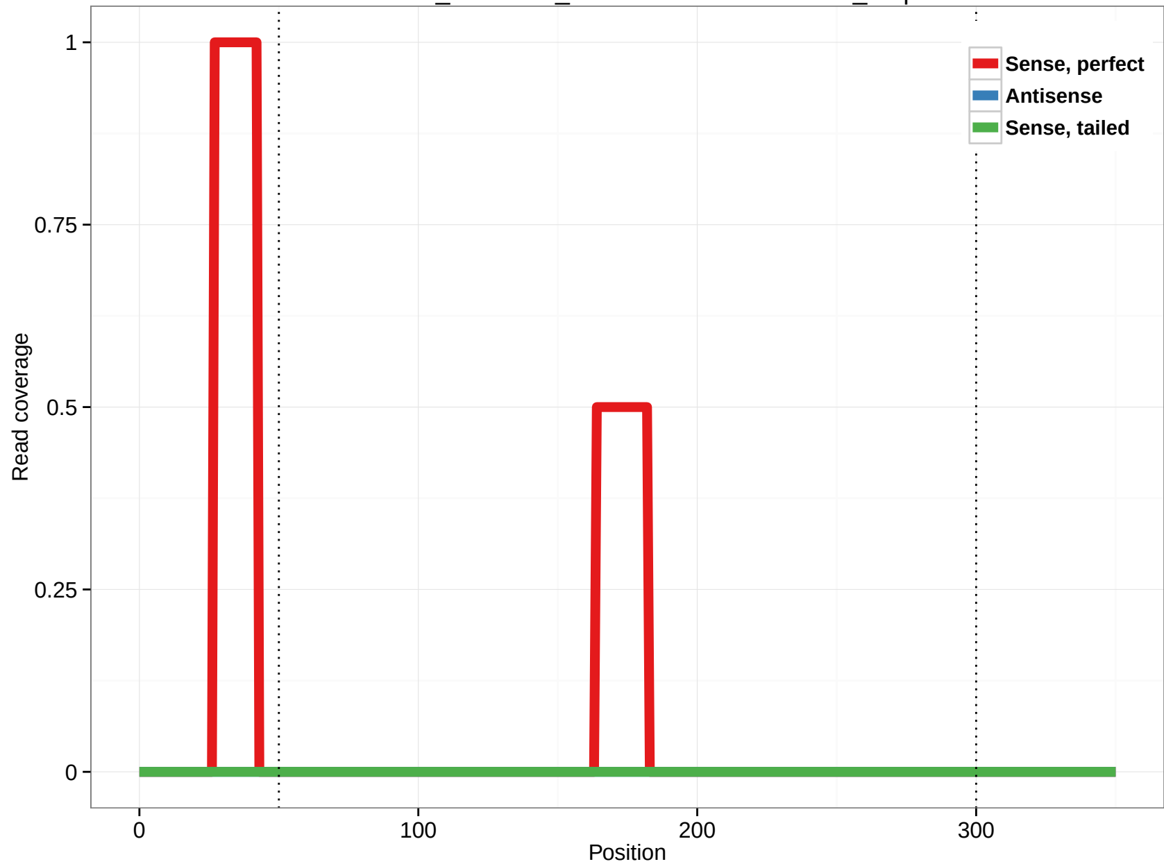
ornAna1_ensGene_ENSOANT00000004680_2.3p
