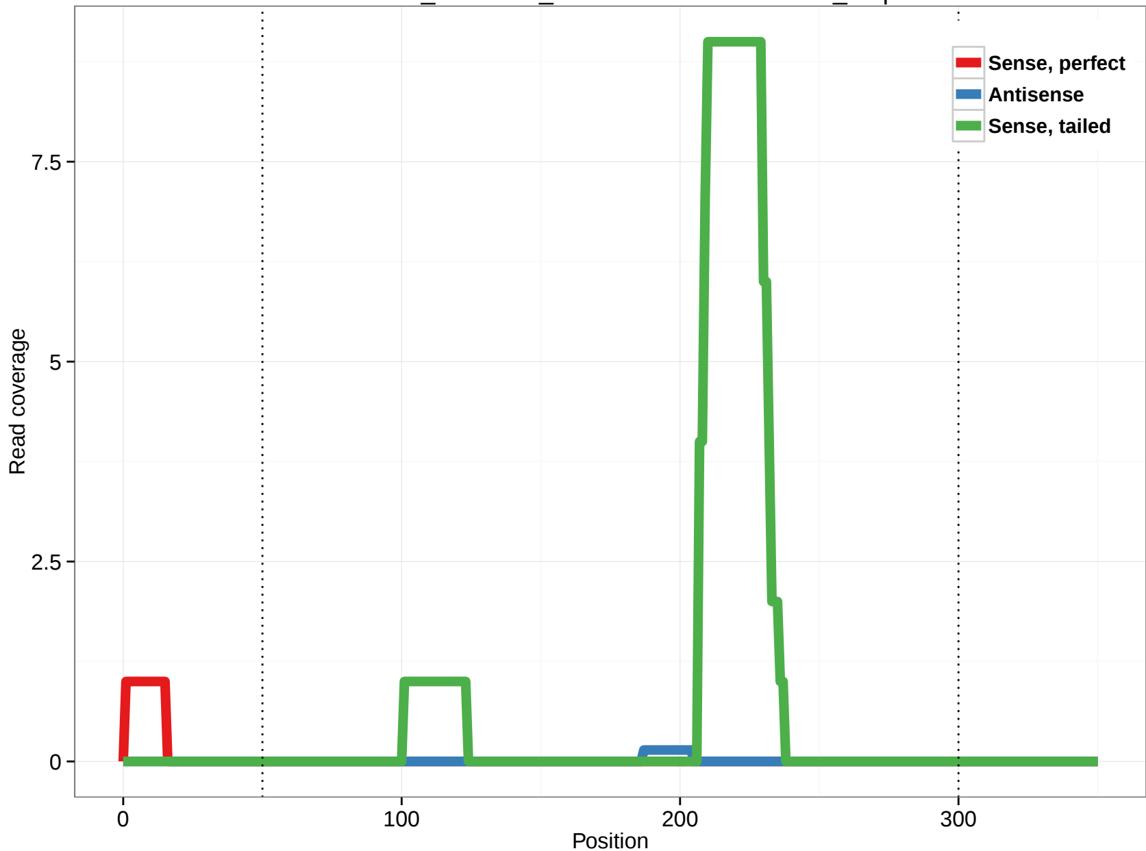
ornAna1_ensGene_ENSOANT00000004559_3.5p
