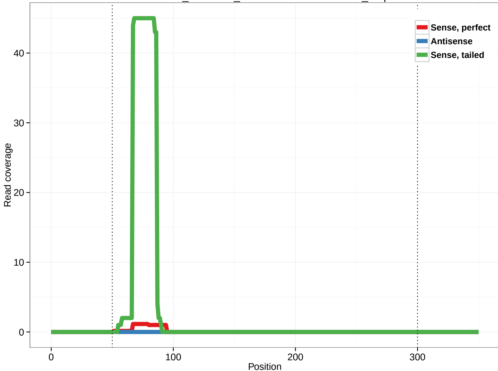
ornAna1_ensGene_ENSOANT00000004544_1.3p
