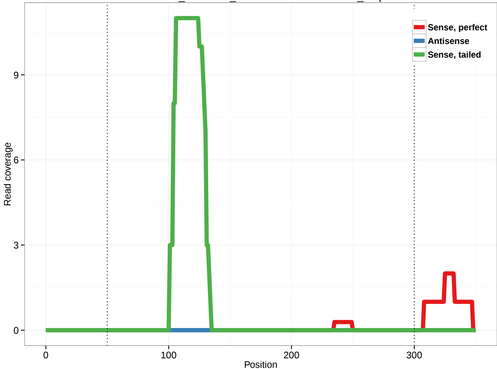
ornAna1_ensGene_ENSOANT00000004480_3.3p
