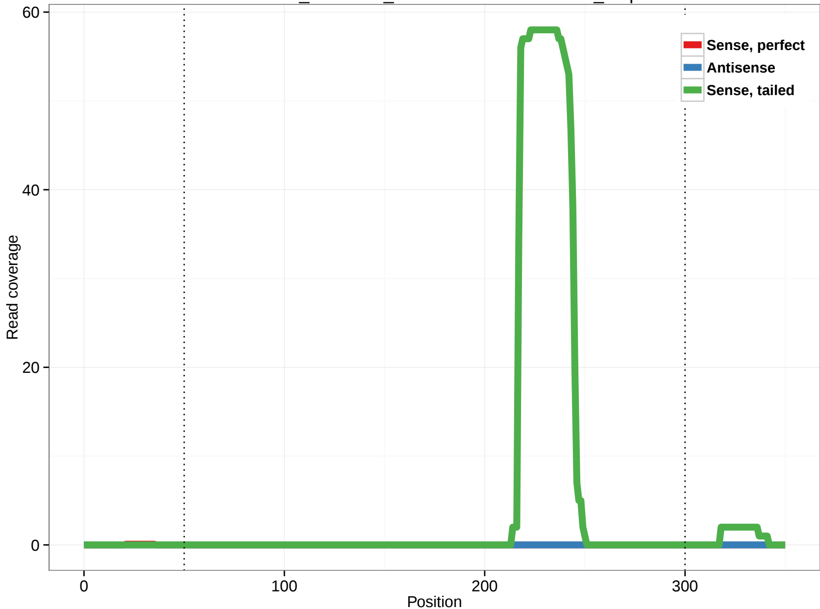
ornAna1_ensGene_ENSOANT00000004420_9.5p
