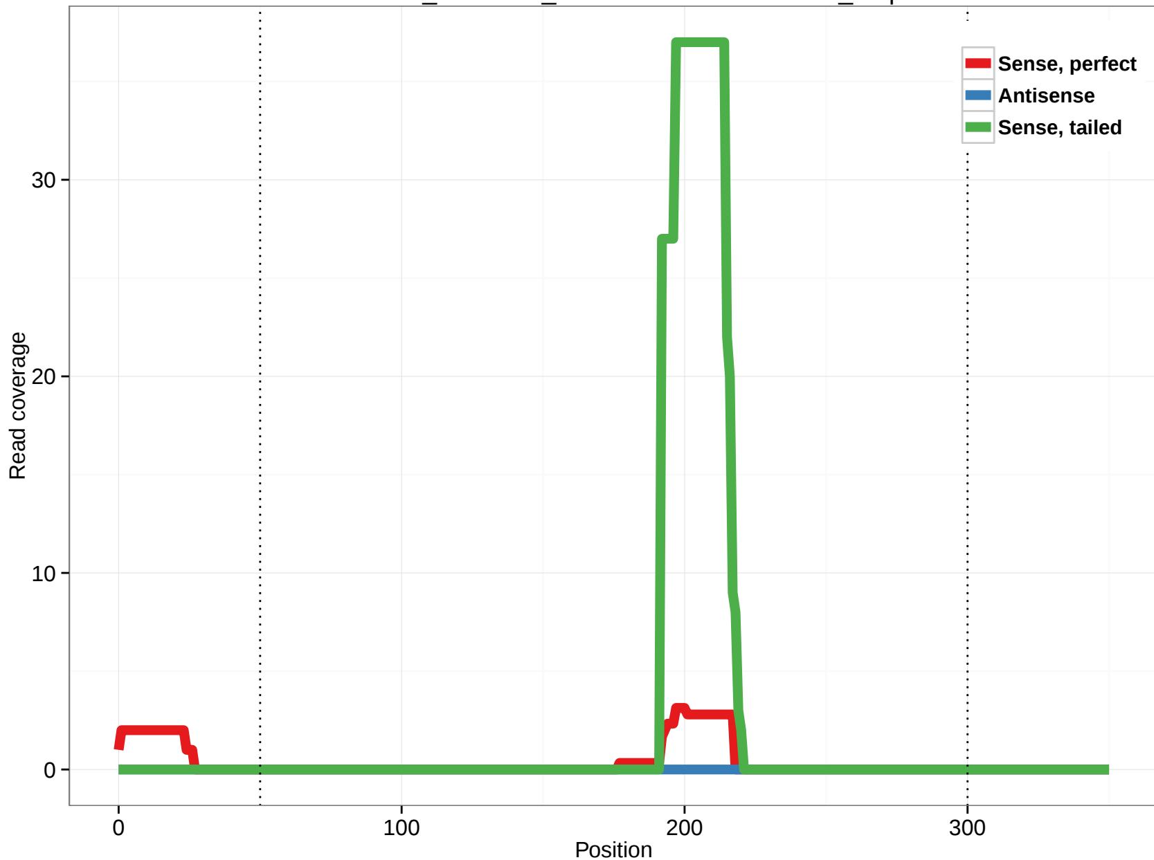
ornAna1_ensGene_ENSOANT00000004415_6.5p
