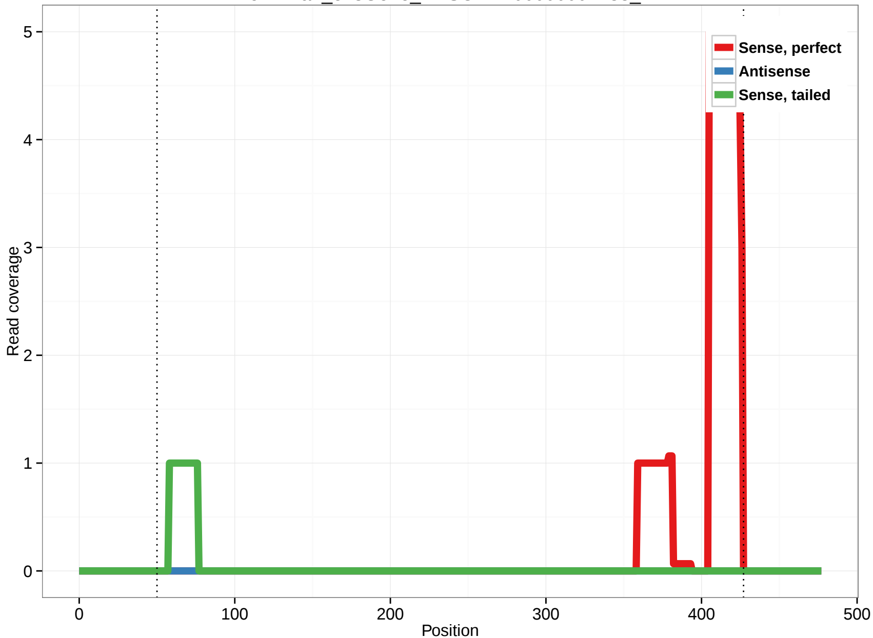
ornAna1_ensGene_ENSOANT00000004288_1
