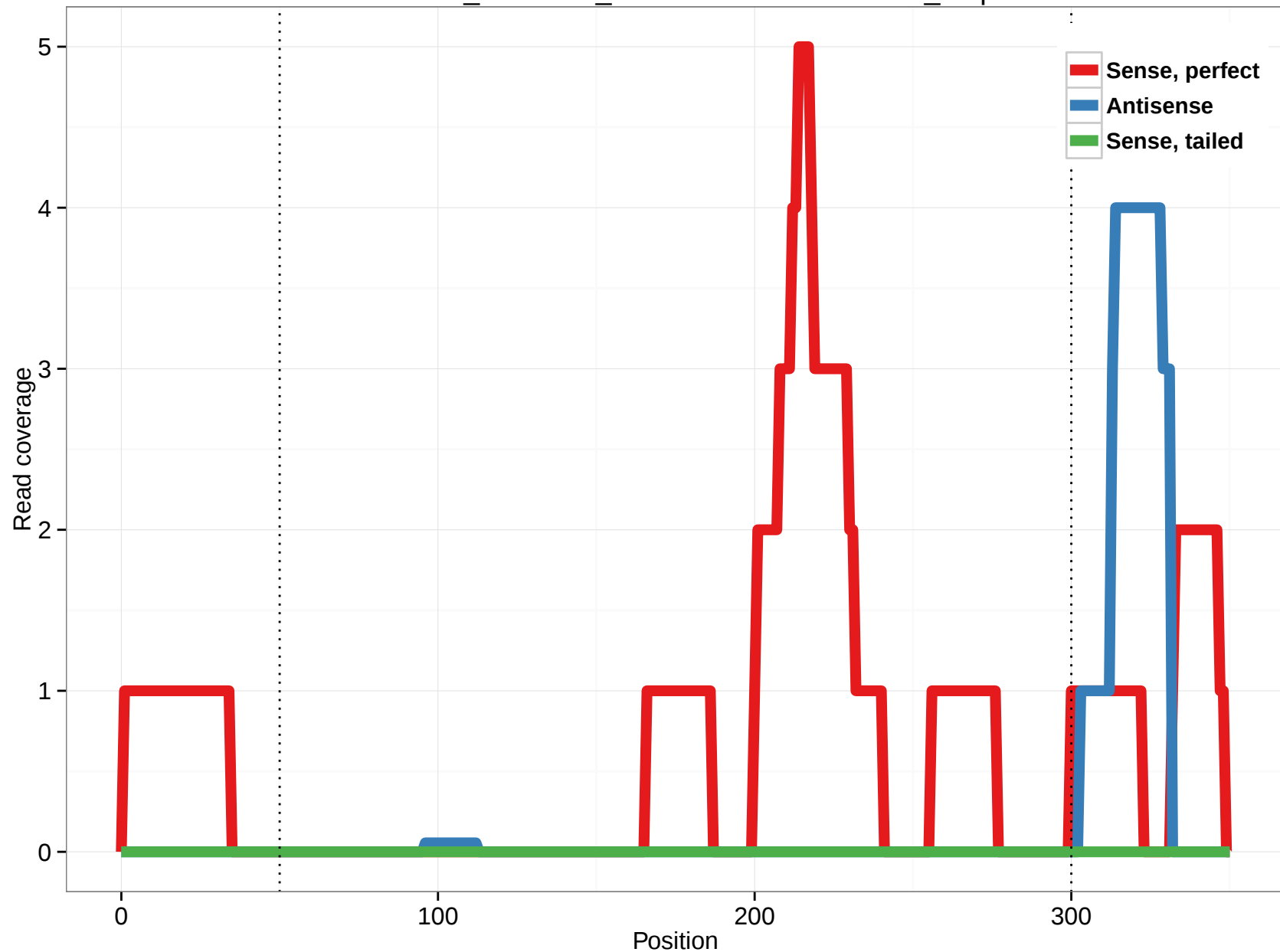
ornAna1_ensGene_ENSOANT00000004279_2.3p
