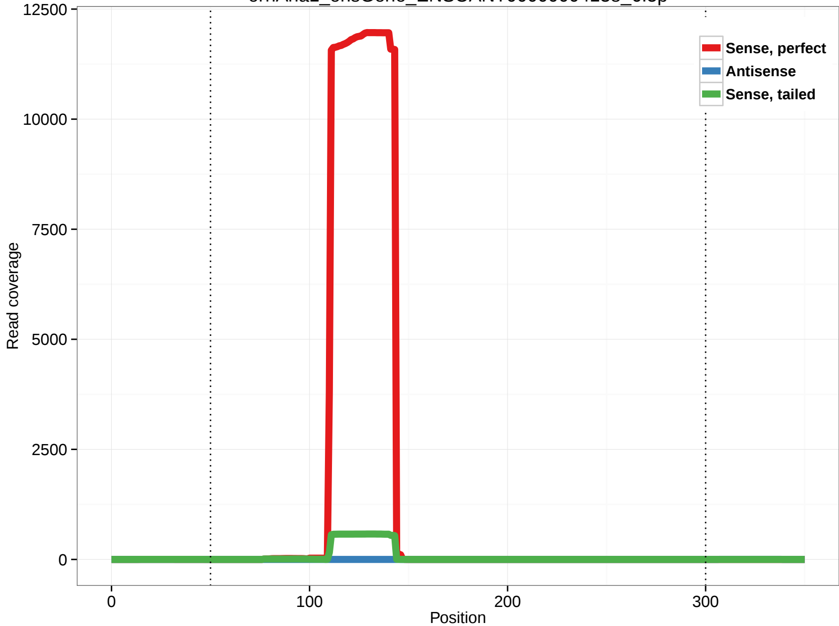
ornAna1_ensGene_ENSOANT00000004138_6.5p
