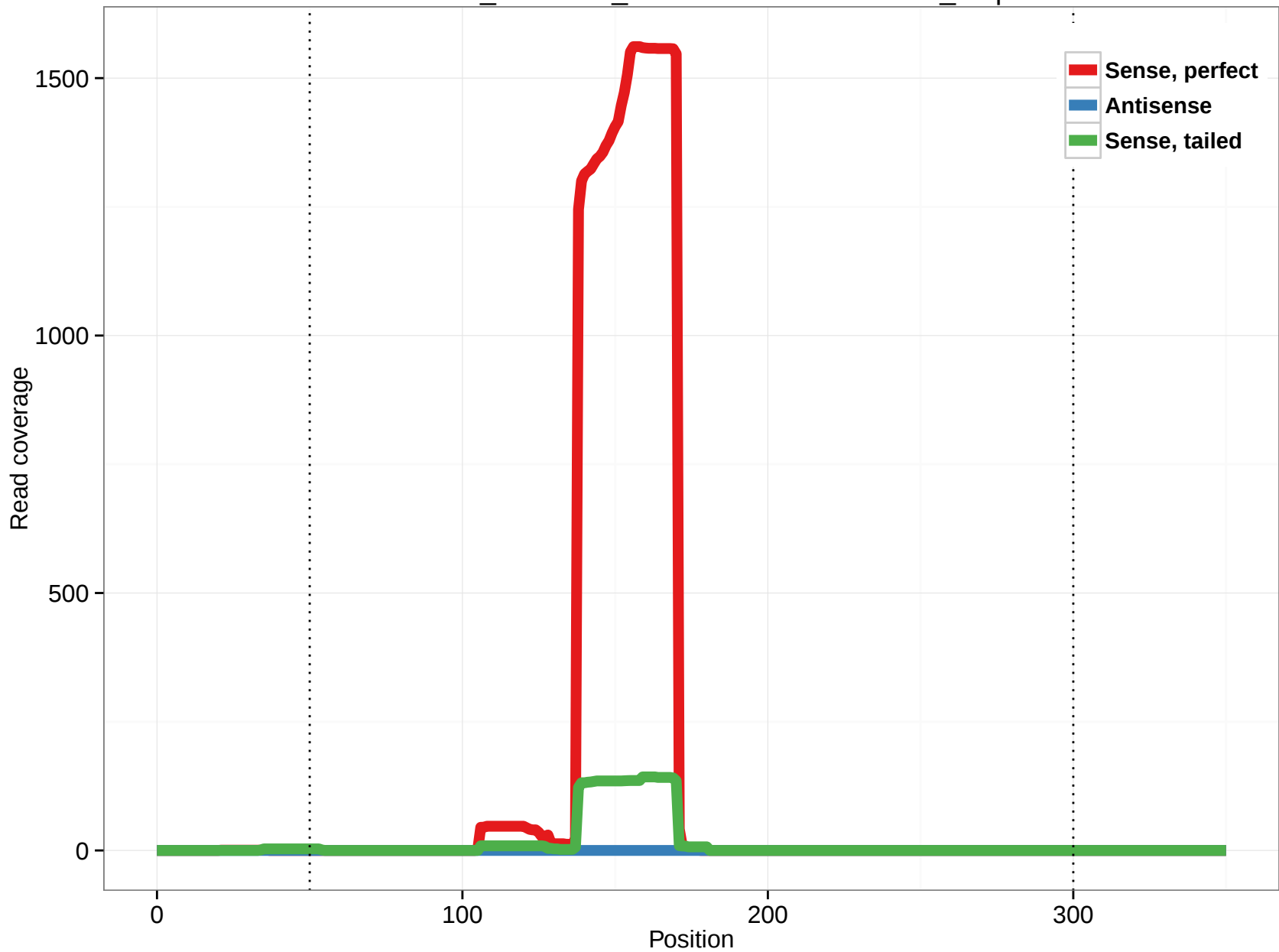
ornAna1_ensGene_ENSOANT00000004138_5.5p
