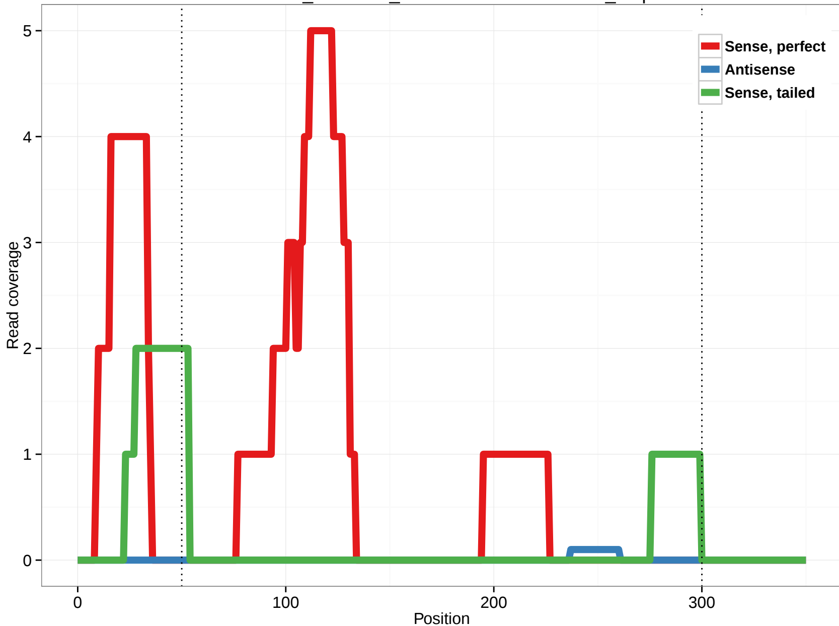
ornAna1_ensGene_ENSOANT00000004136_4.5p
