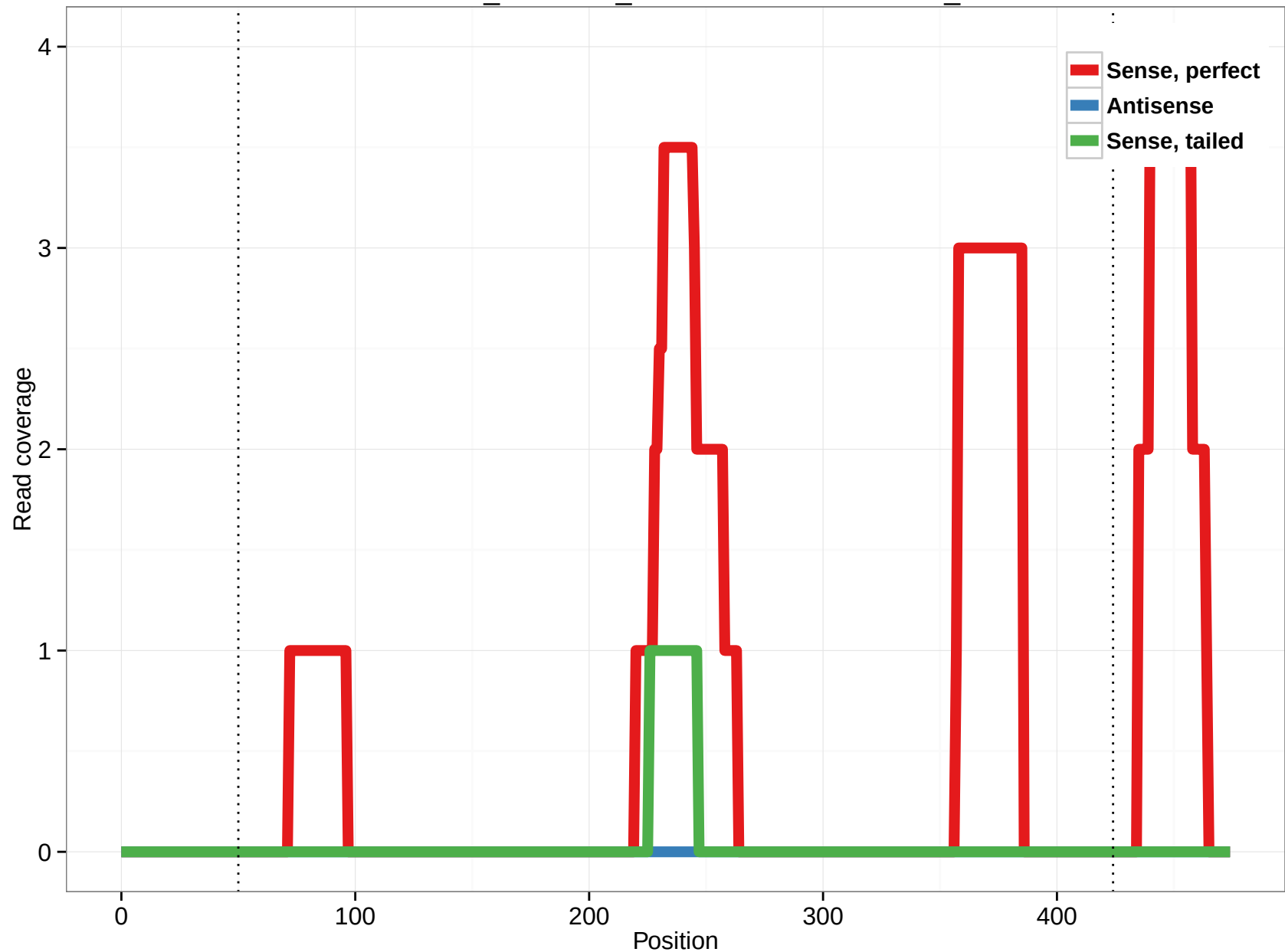
ornAna1_ensGene_ENSOANT00000004116_3
