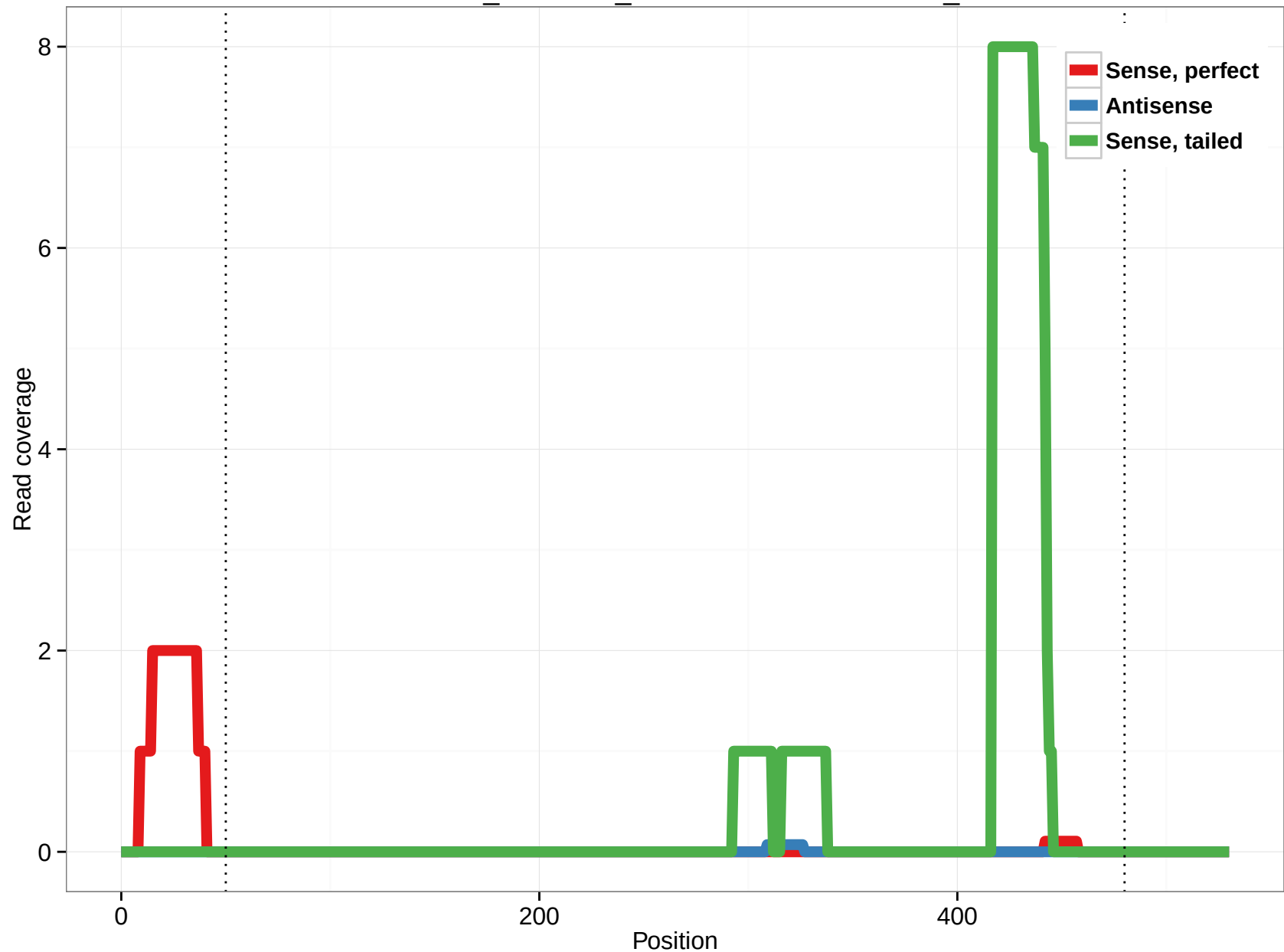
ornAna1_ensGene_ENSOANT00000004039_3
