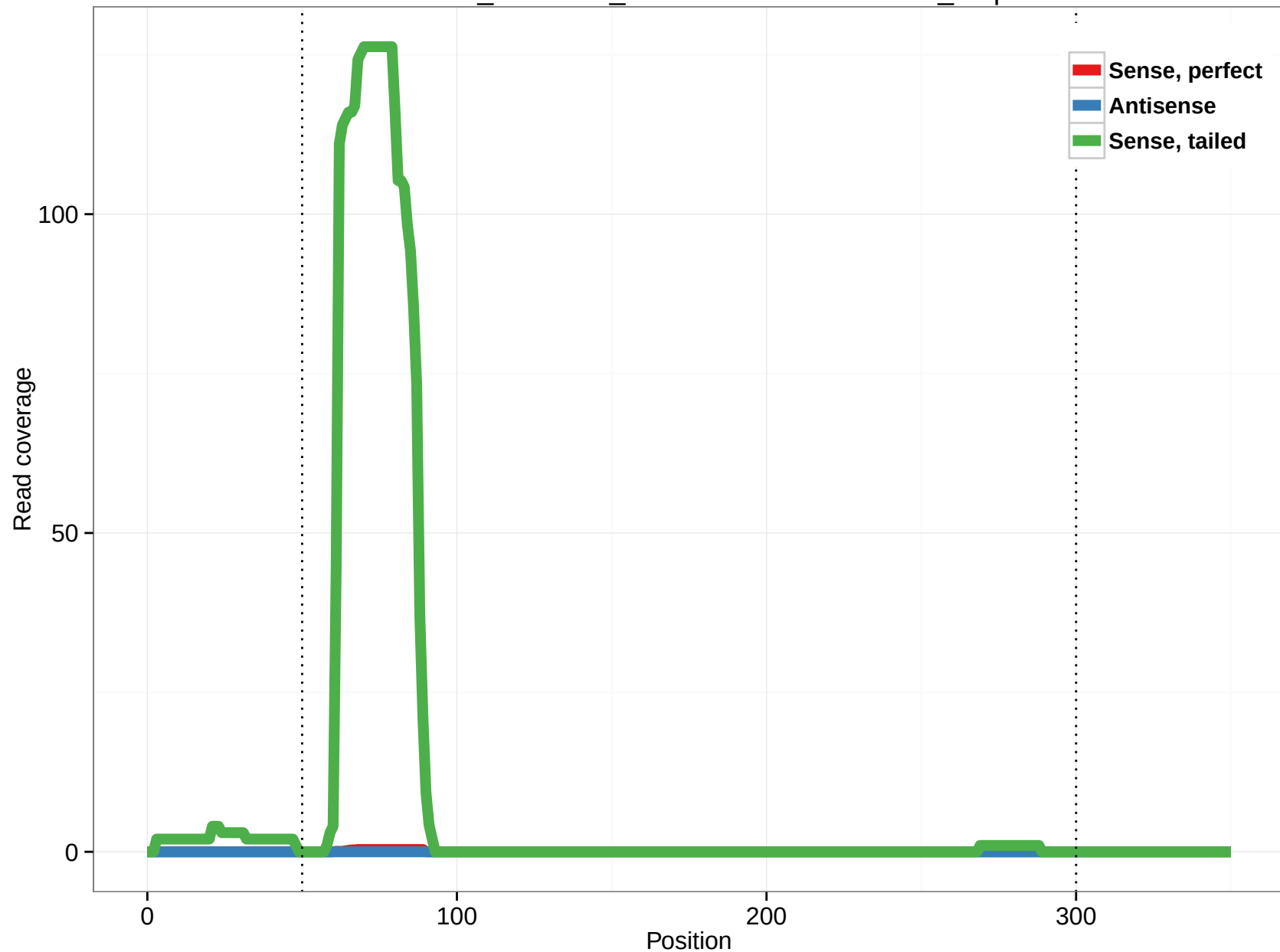
ornAna1_ensGene_ENSOANT00000004007_6.3p
