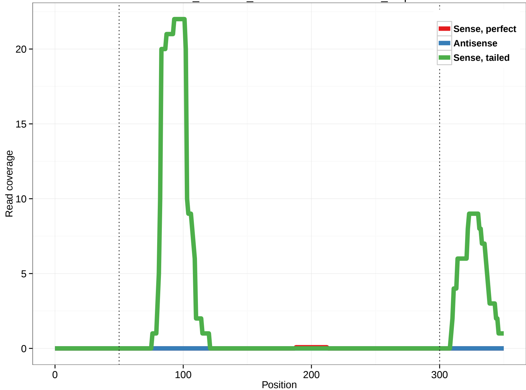
ornAna1_ensGene_ENSOANT00000003990_5.5p
