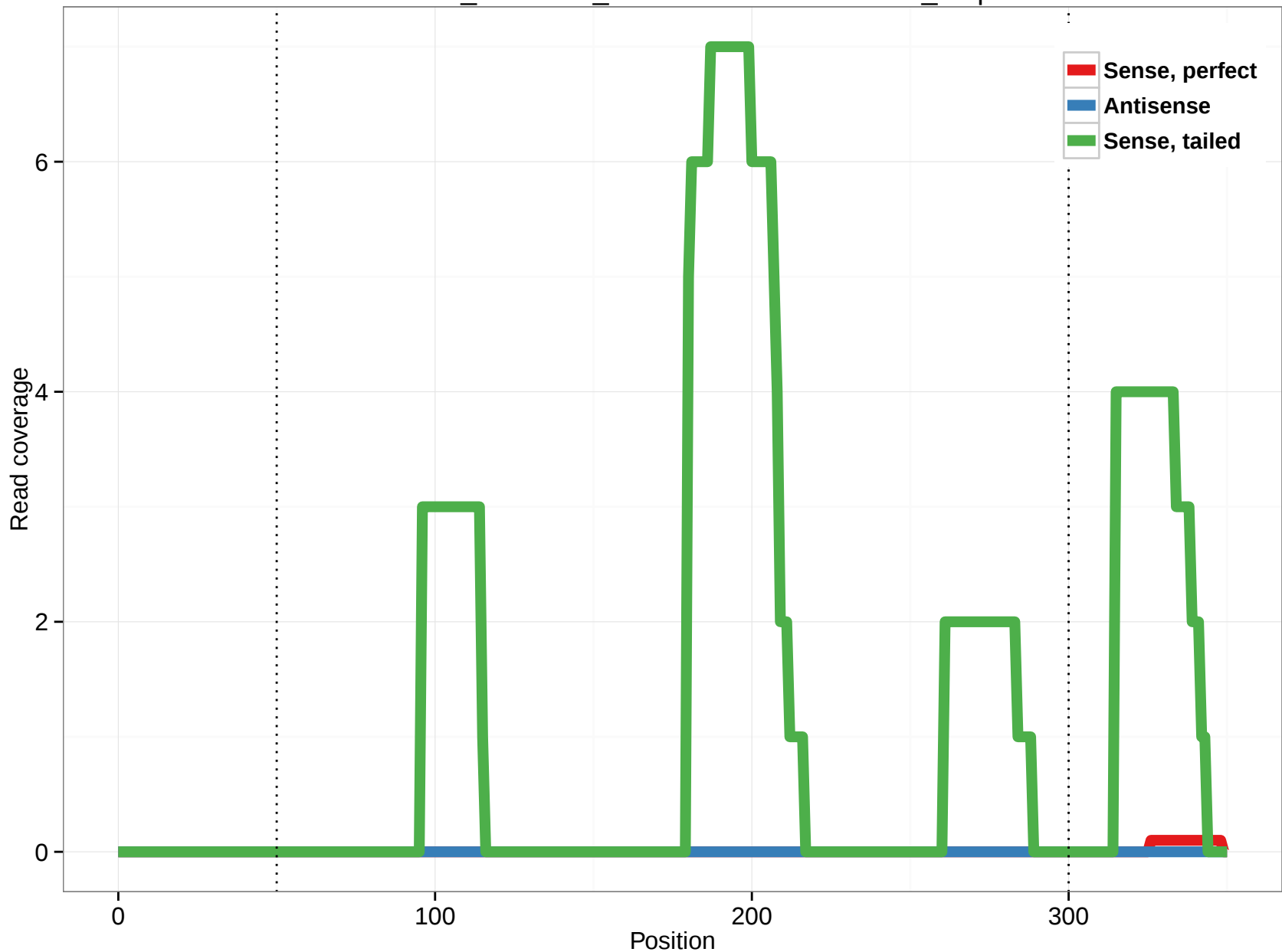
ornAna1_ensGene_ENSOANT00000003947_6.5p
