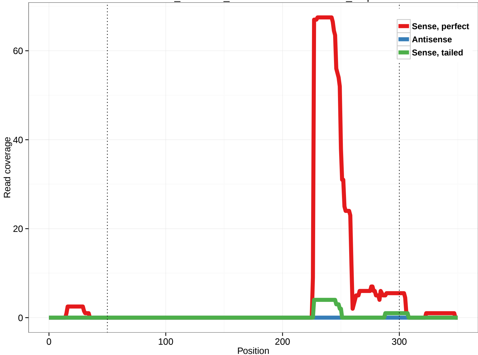
ornAna1_ensGene_ENSOANT00000003837_6.5p
