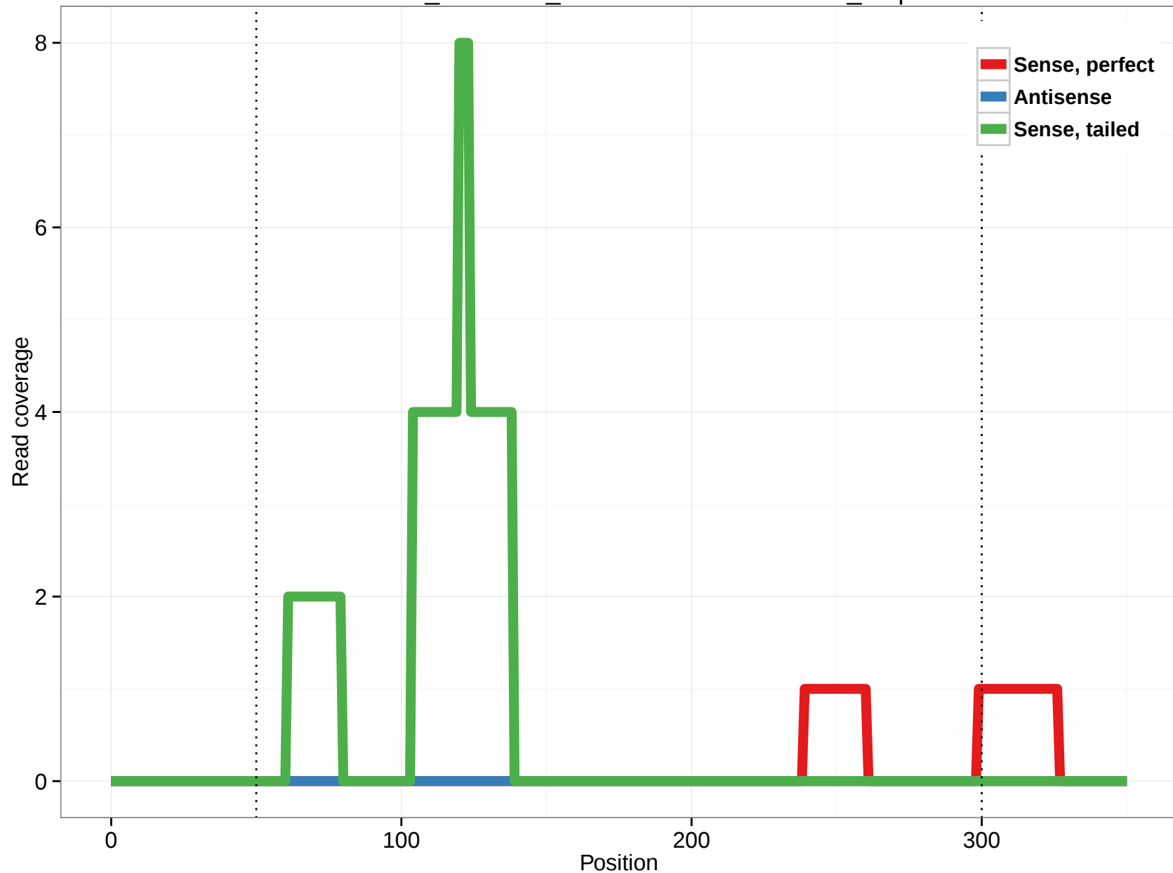
ornAna1_ensGene_ENSOANT00000003796_3.3p
