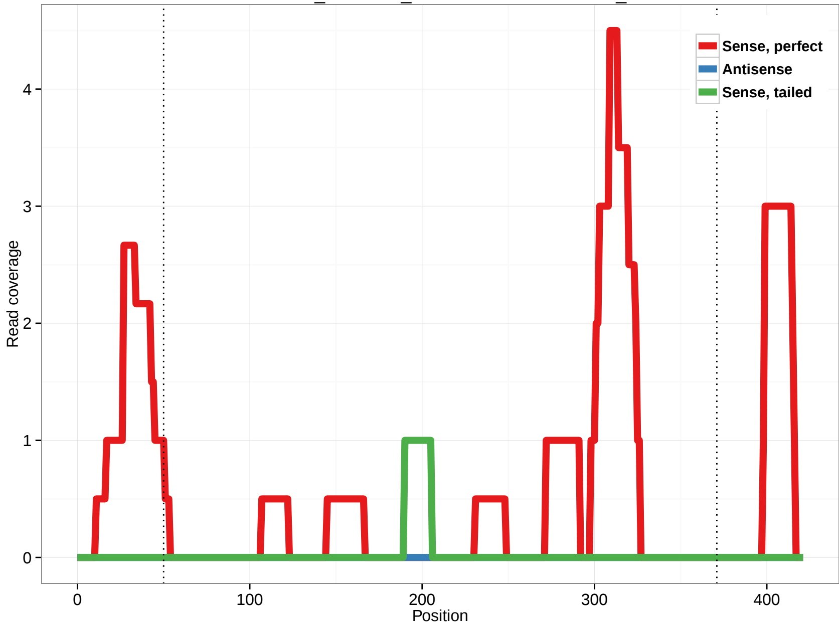
ornAna1_ensGene_ENSOANT00000003789_3
