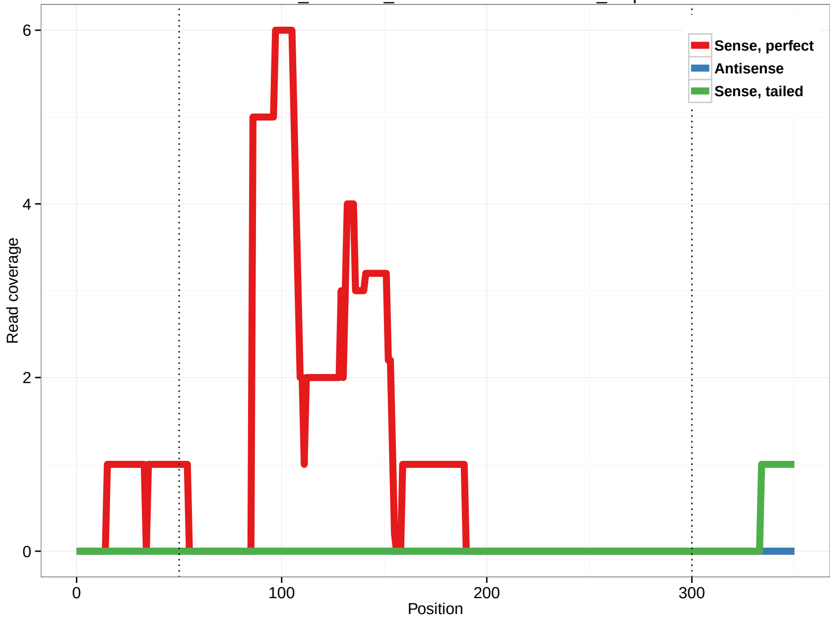
ornAna1_ensGene_ENSOANT00000003787_2.3p
