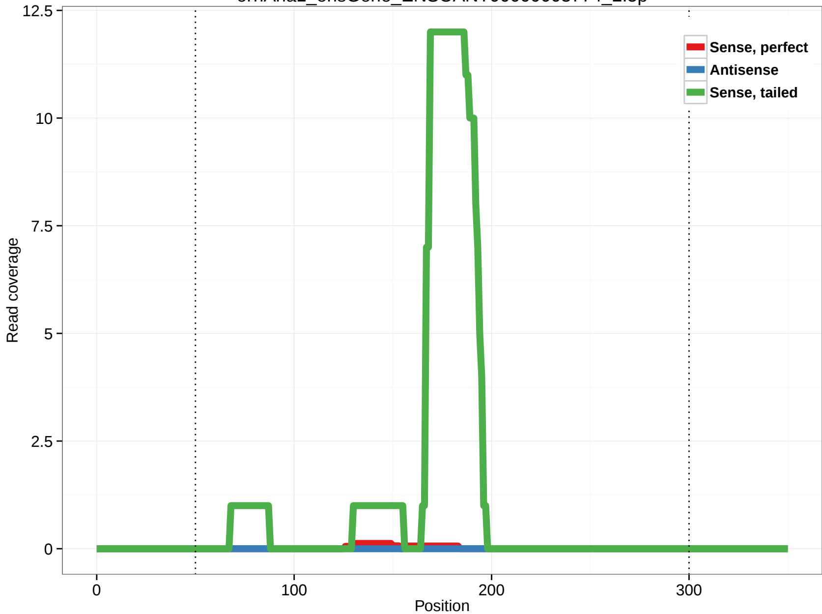
ornAna1_ensGene_ENSOANT00000003774_2.5p
