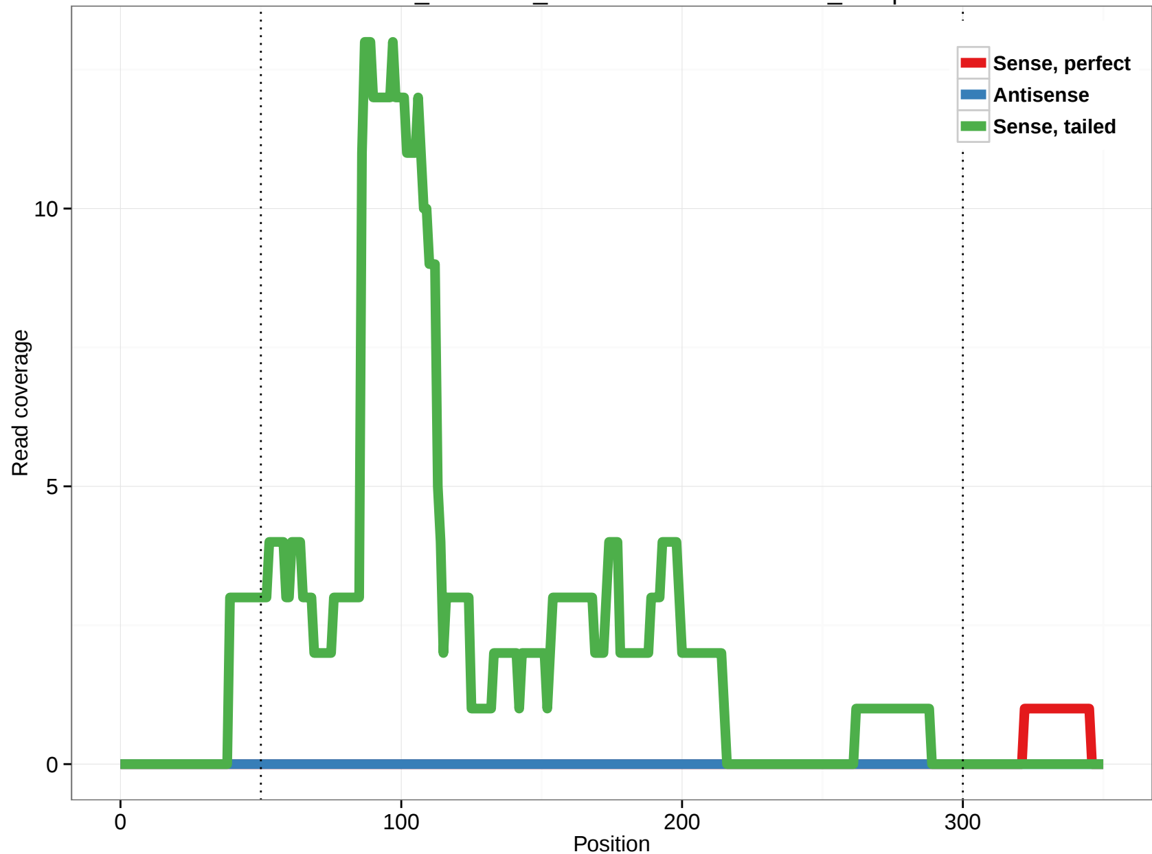
ornAna1_ensGene_ENSOANT00000003700_36.3p
