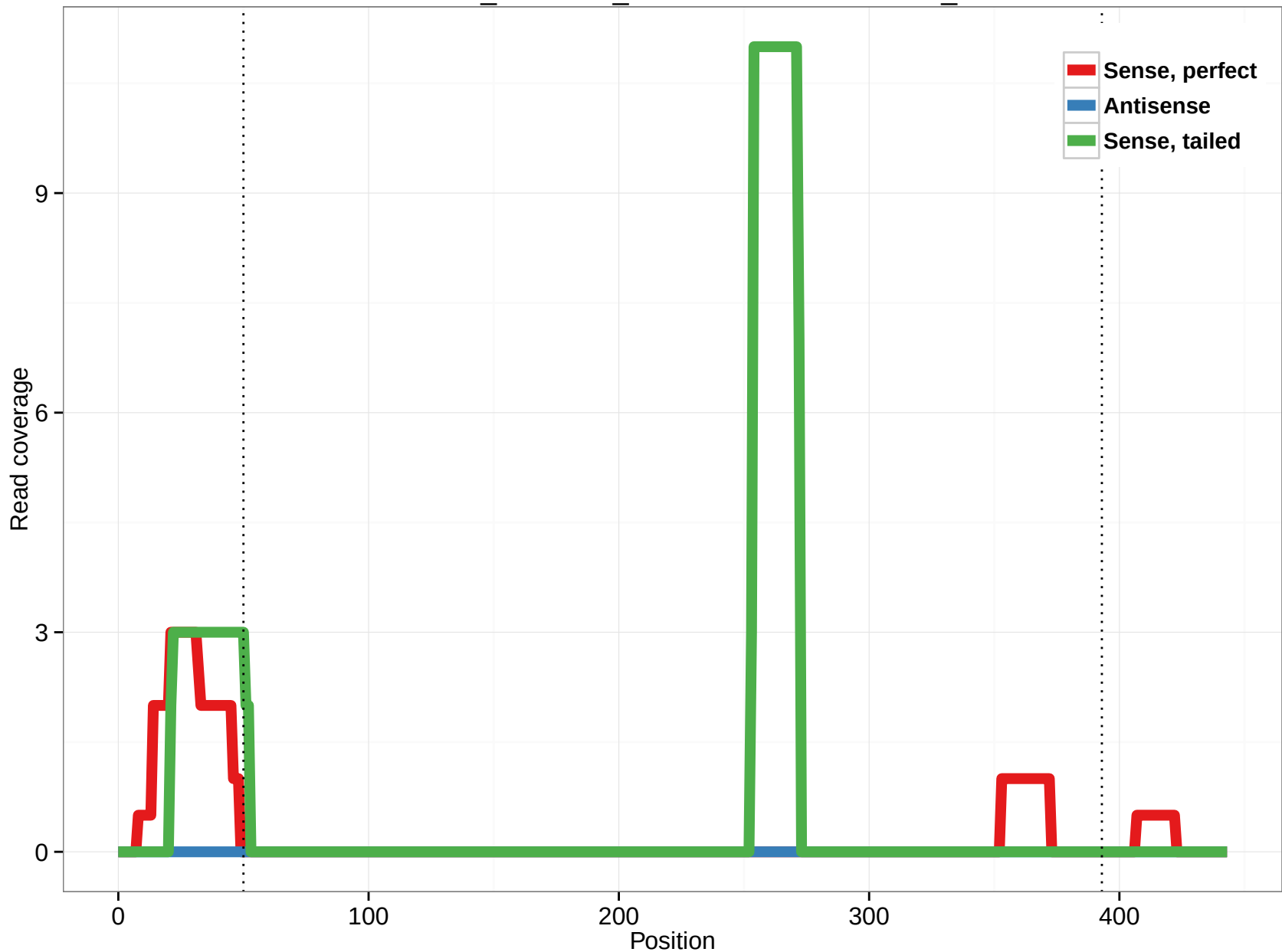
ornAna1_ensGene_ENSOANT00000003675_8
