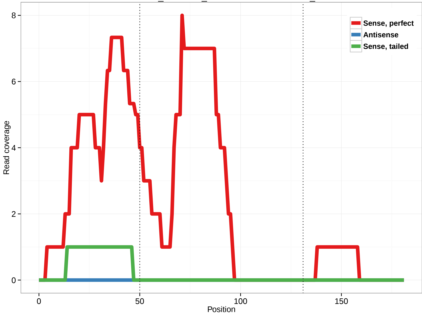
ornAna1_ensGene_ENSOANT00000003604_3
