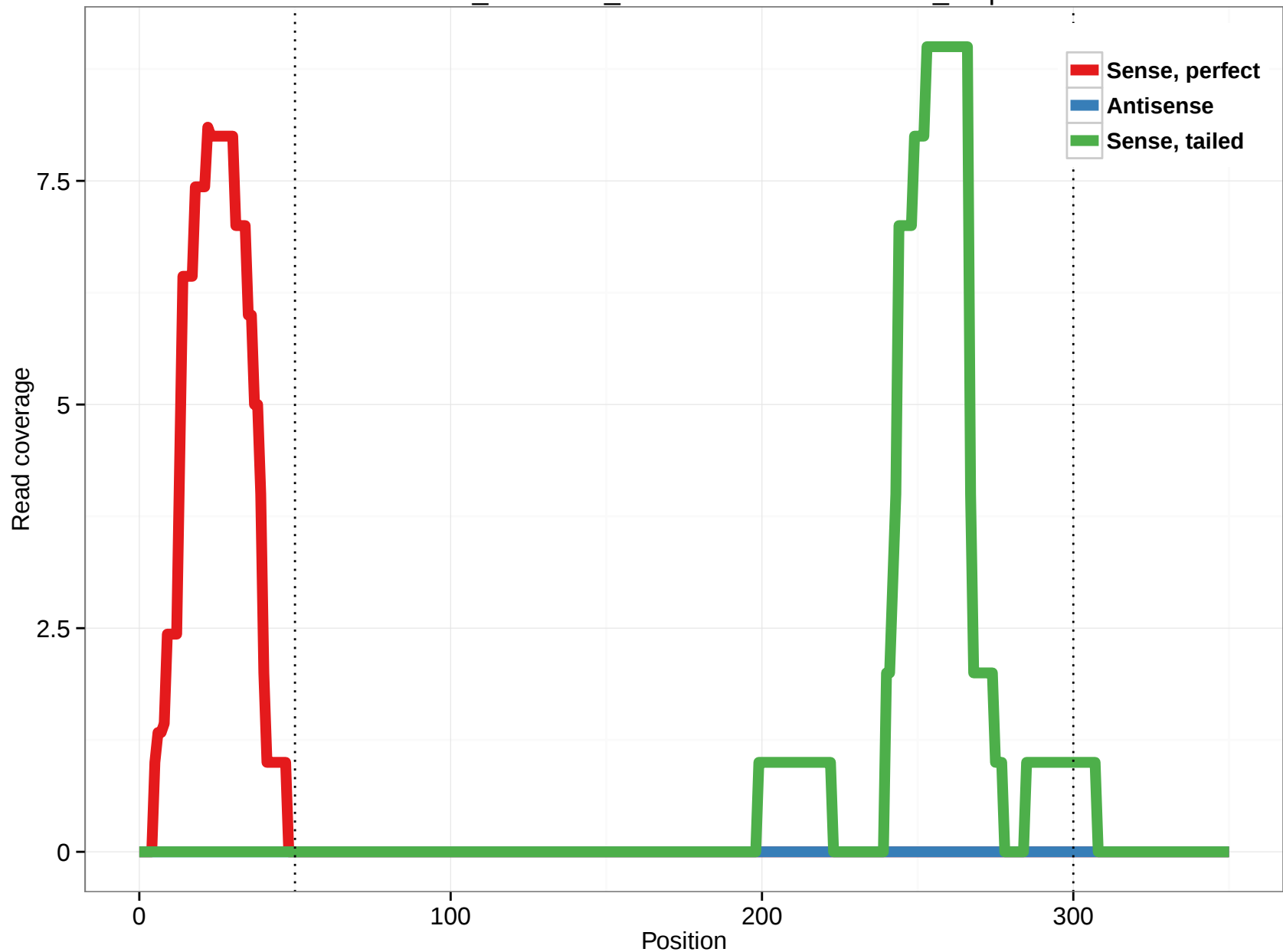
ornAna1_ensGene_ENSOANT00000003570_2.5p
