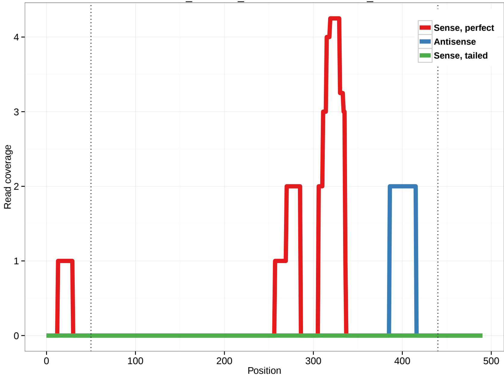
ornAna1_ensGene_ENSOANT00000003490_11
