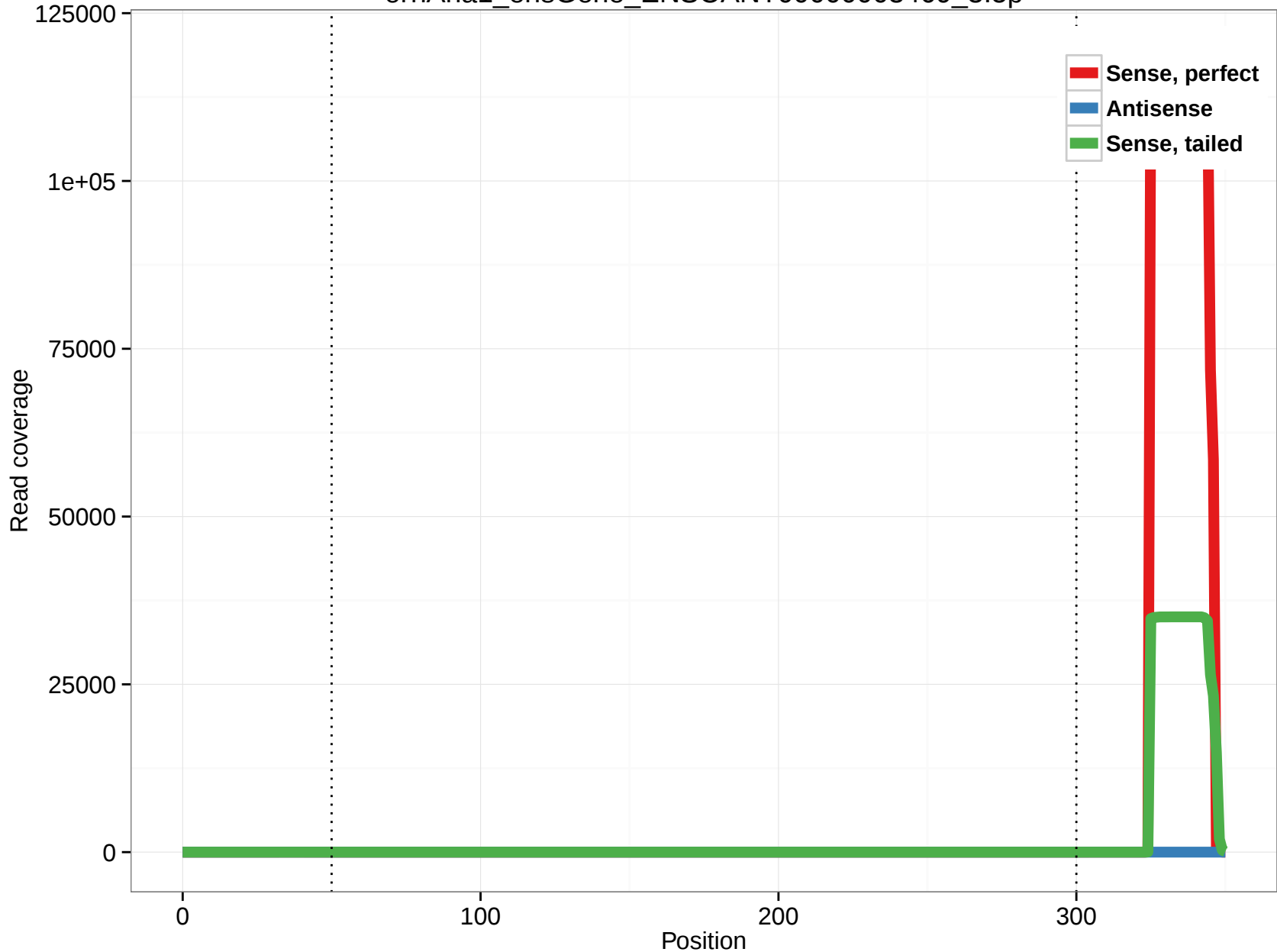
ornAna1_ensGene_ENSOANT00000003469_3.5p
