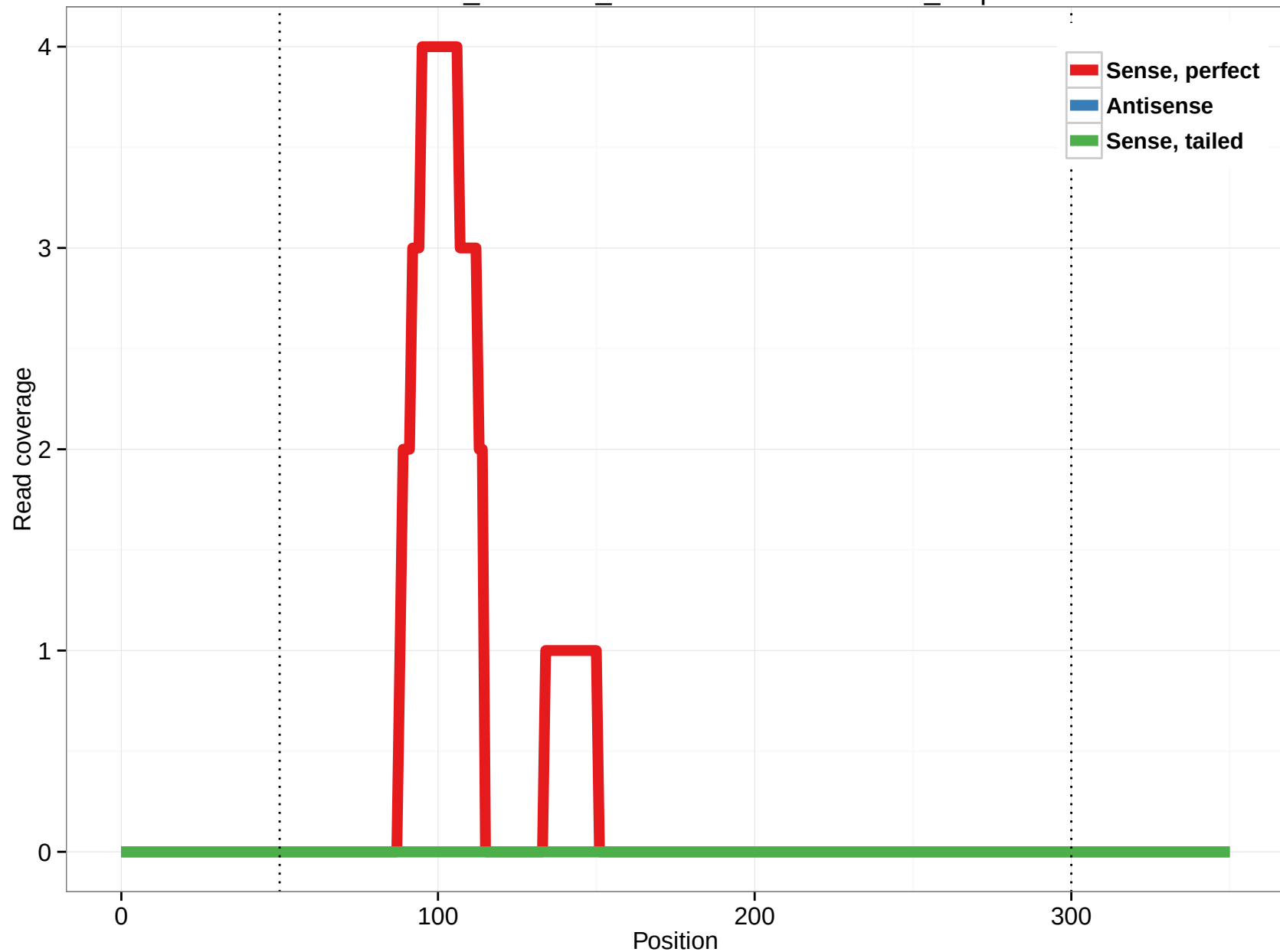
ornAna1_ensGene_ENSOANT00000003424_2.3p
