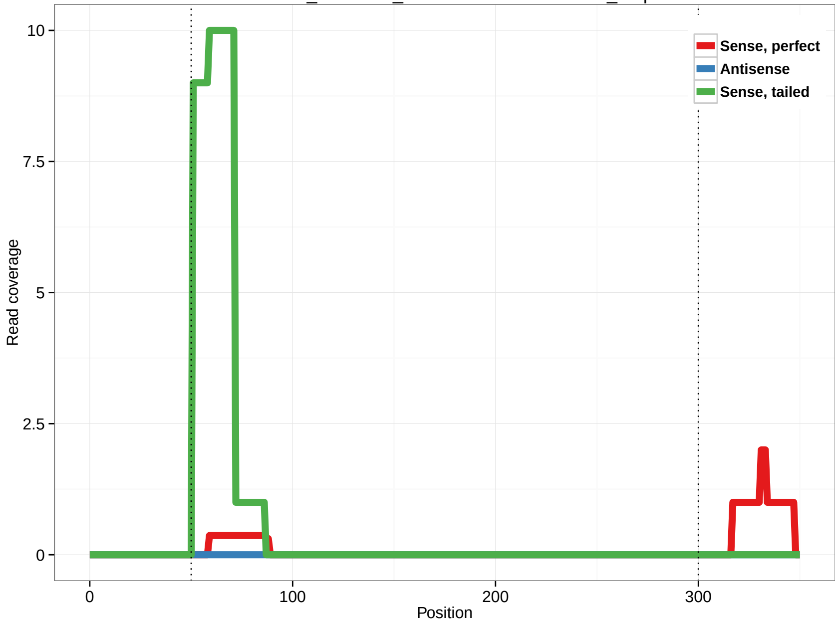
ornAna1_ensGene_ENSOANT00000003390_5.3p
