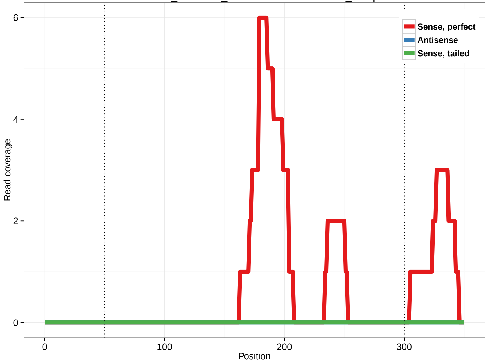
ornAna1_ensGene_ENSOANT00000003380_11.3p
