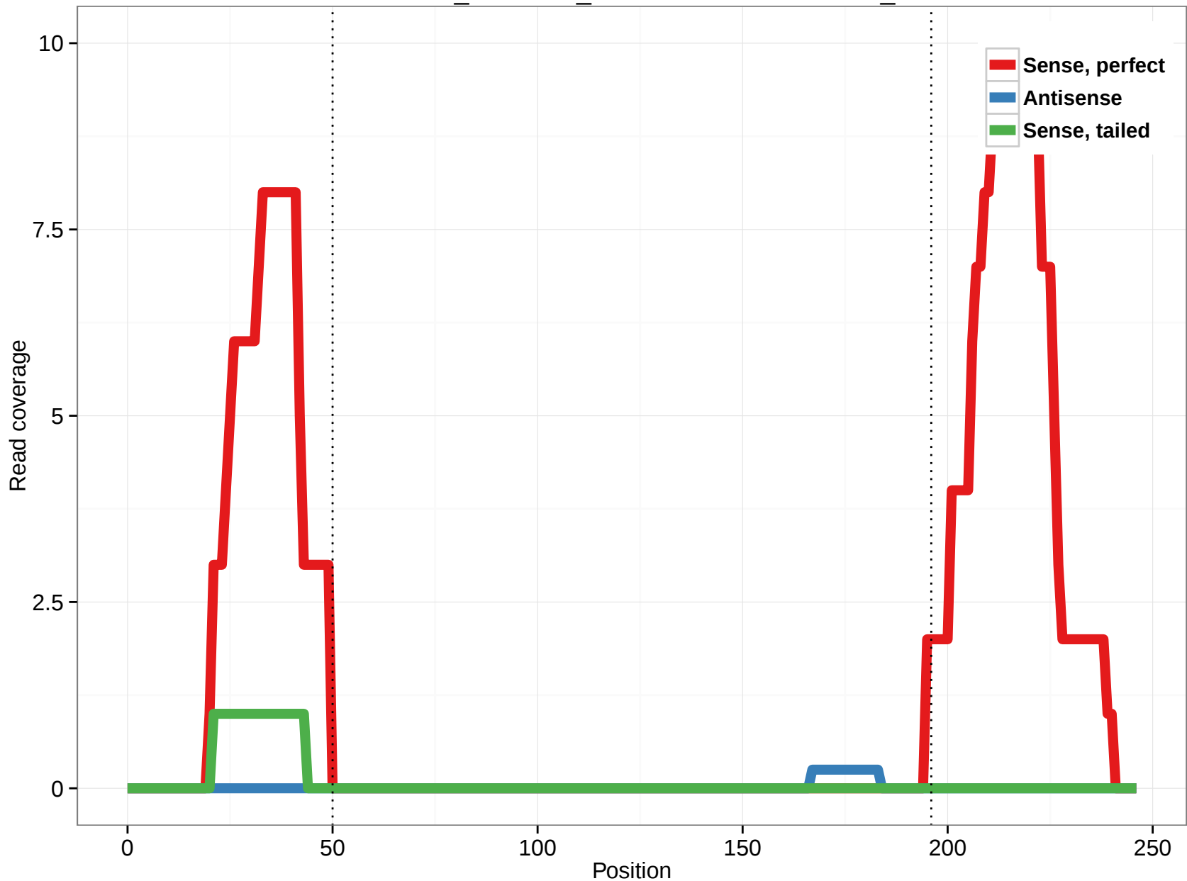
ornAna1_ensGene_ENSOANT00000003355_6
