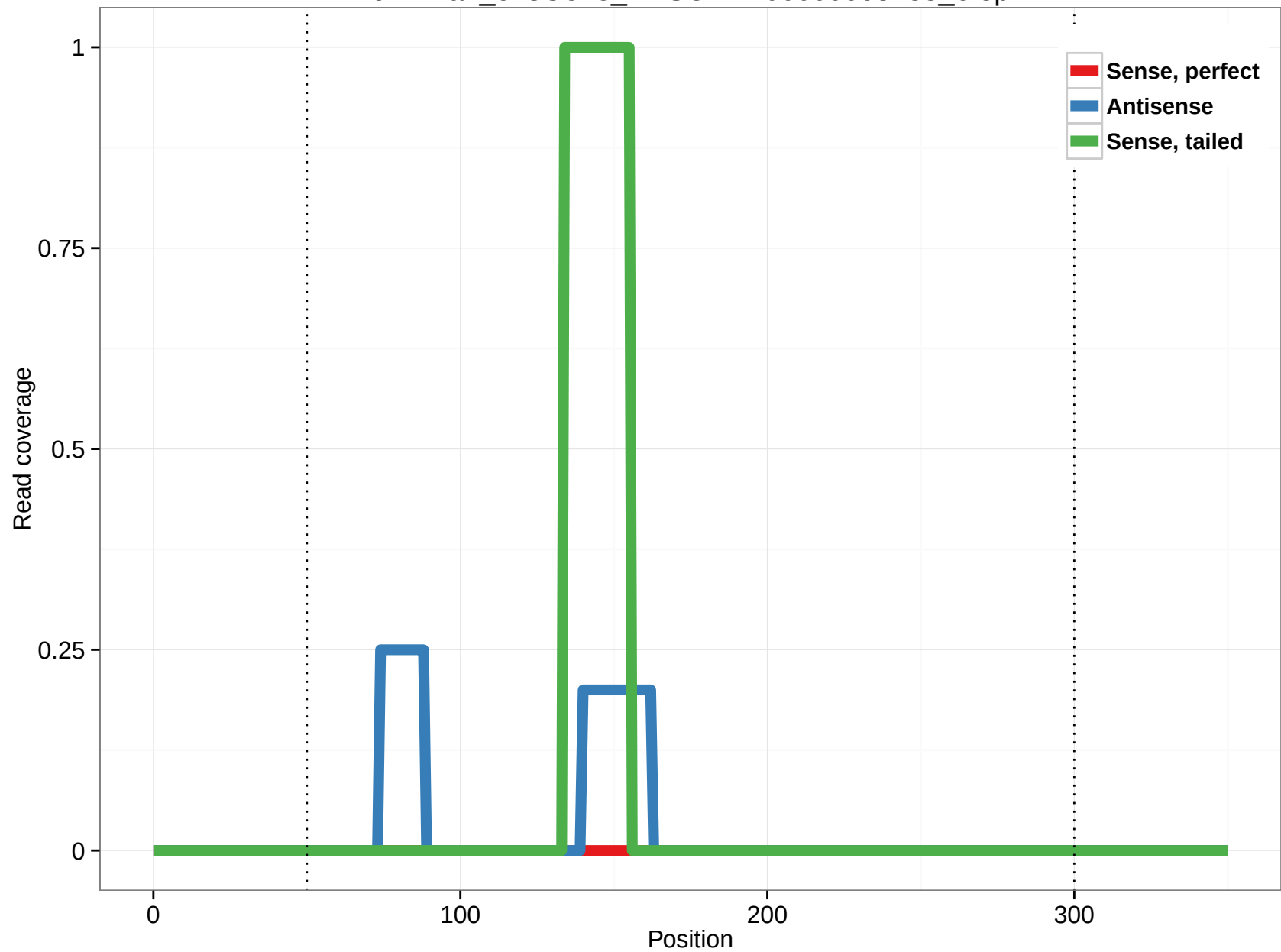
ornAna1_ensGene_ENSOANT00000003288_6.3p
