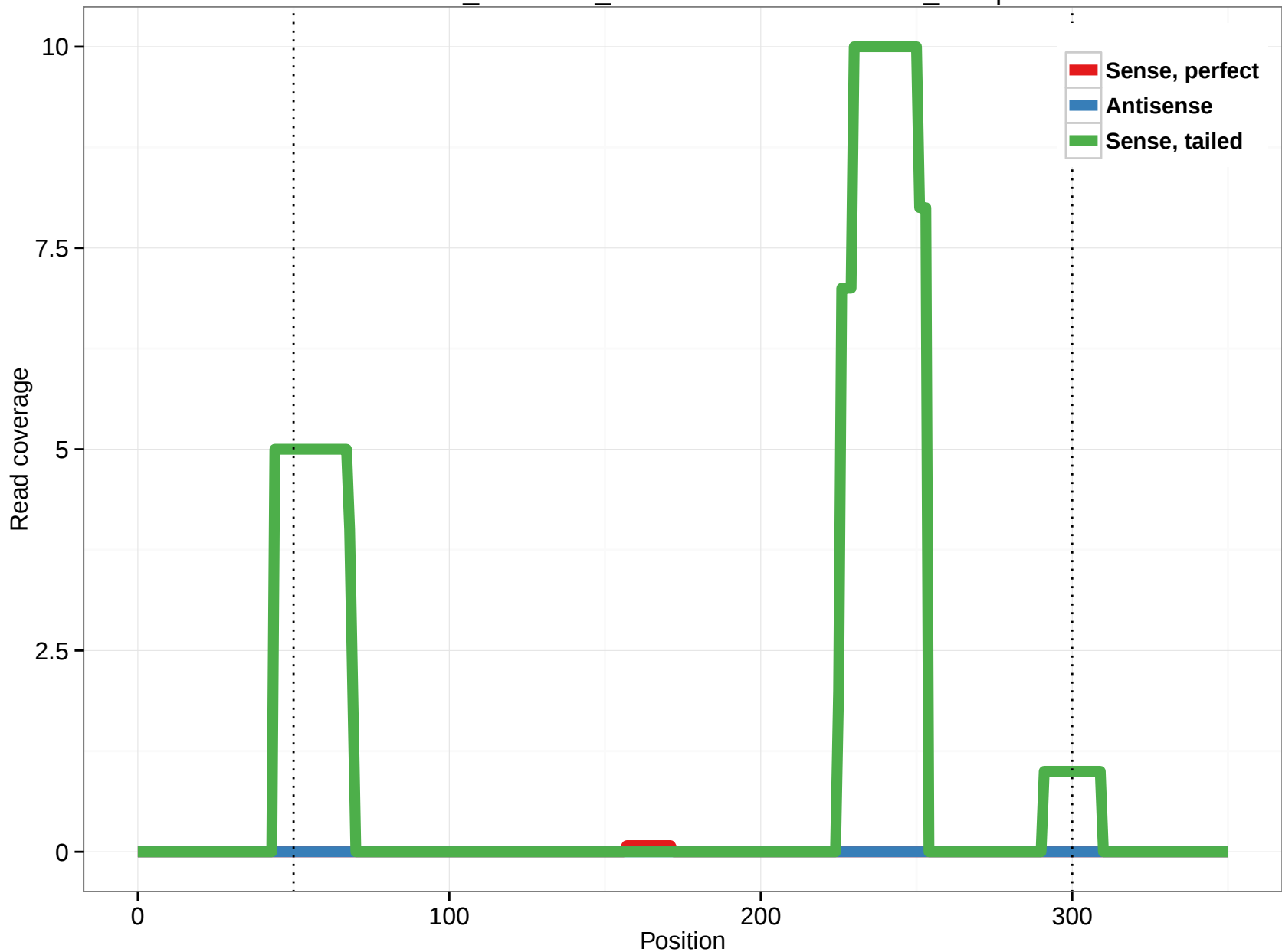
ornAna1_ensGene_ENSOANT00000003179_19.3p
