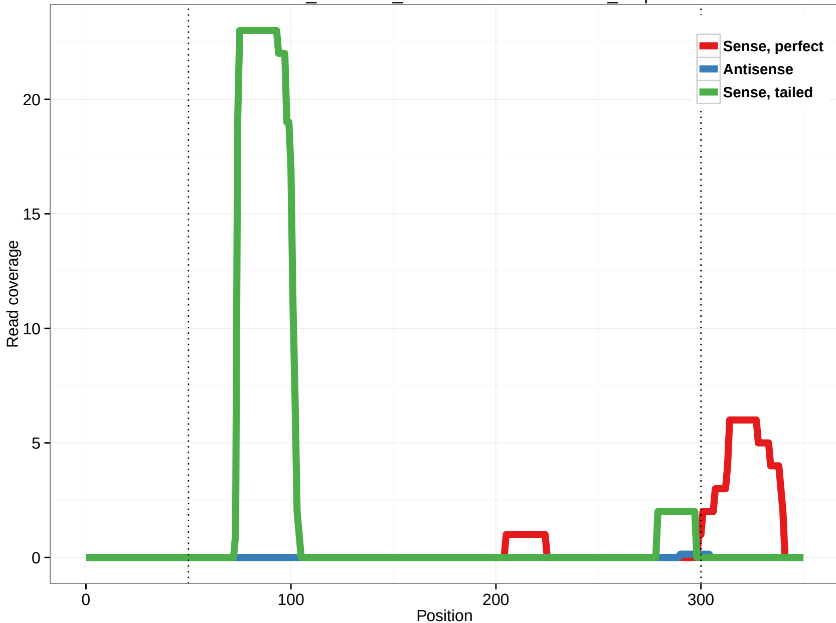
ornAna1_ensGene_ENSOANT00000003148_1.3p
