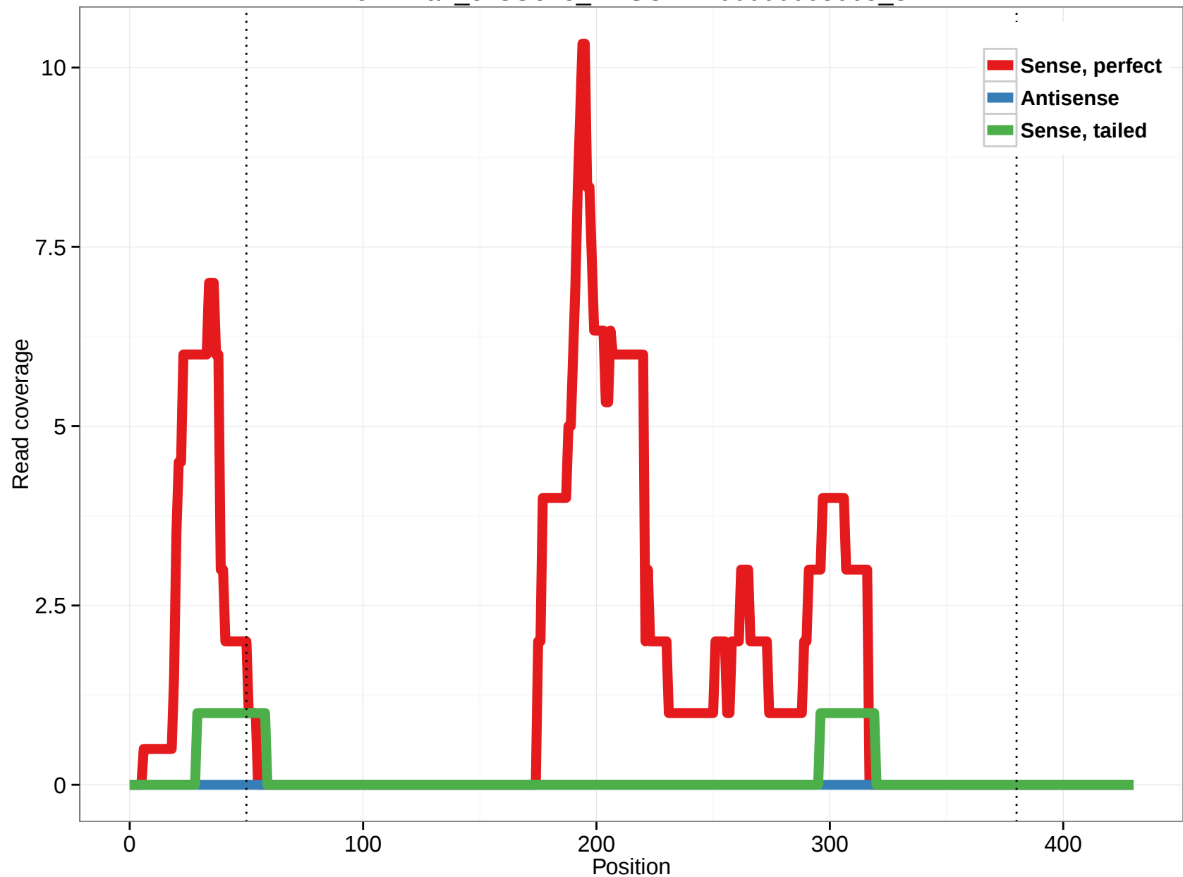
ornAna1_ensGene_ENSOANT00000003065_3
