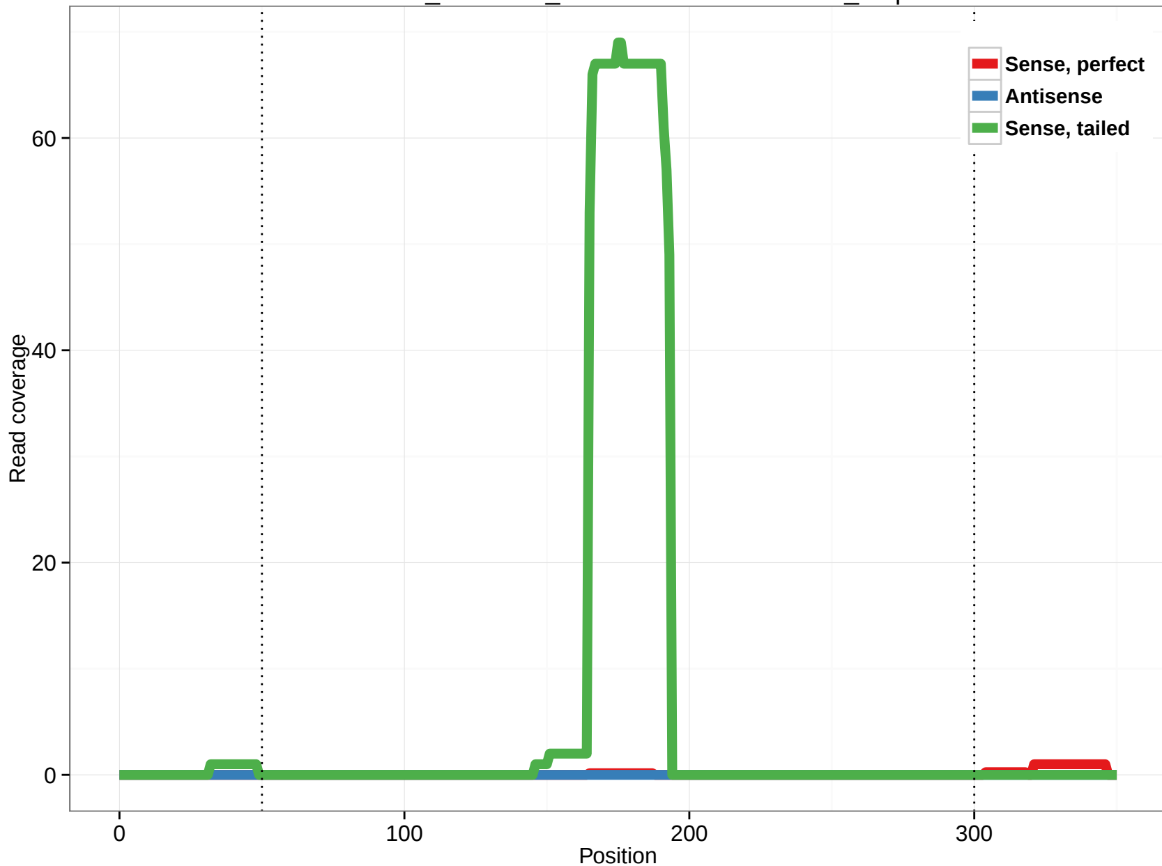
ornAna1_ensGene_ENSOANT00000003058_1.3p
