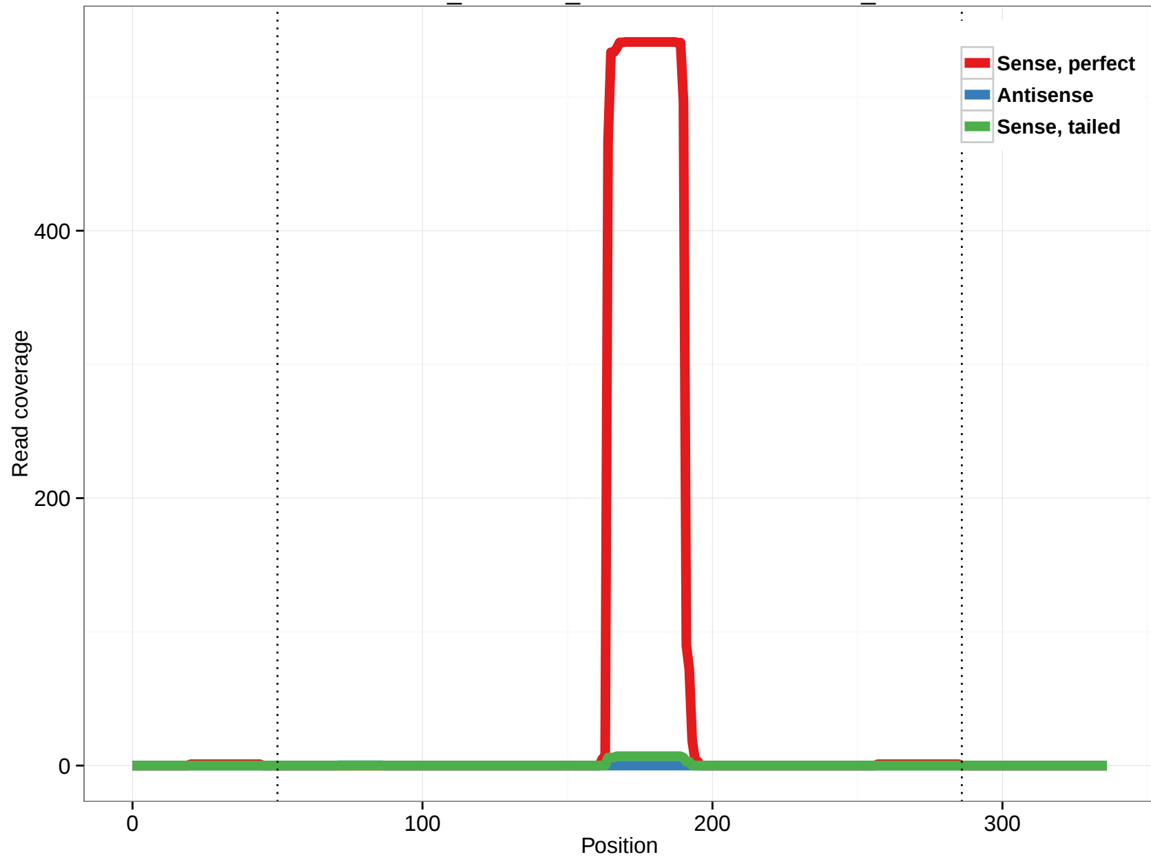
ornAna1_ensGene_ENSOANT00000003044_4
