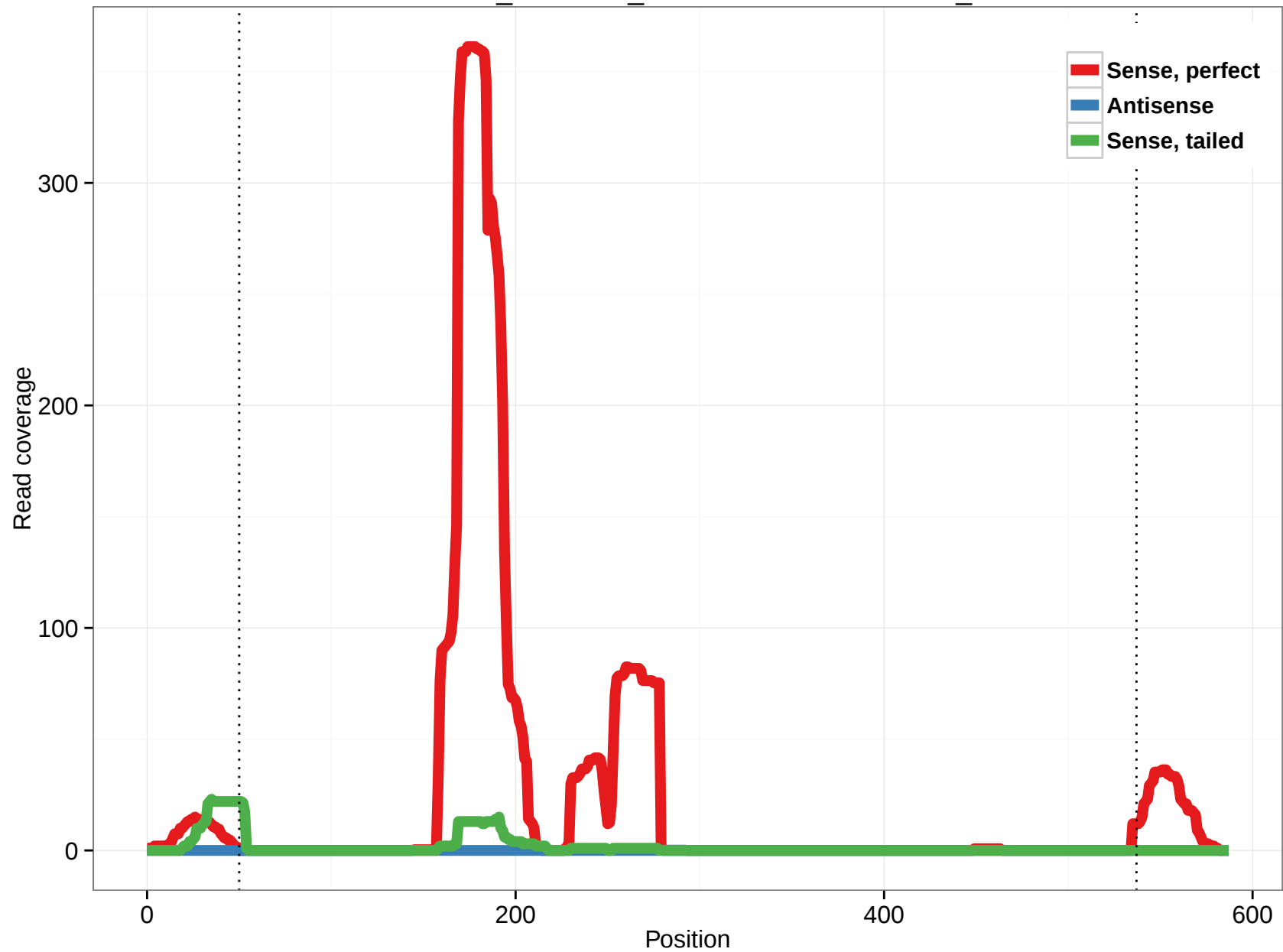
ornAna1_ensGene_ENSOANT00000002991_4
