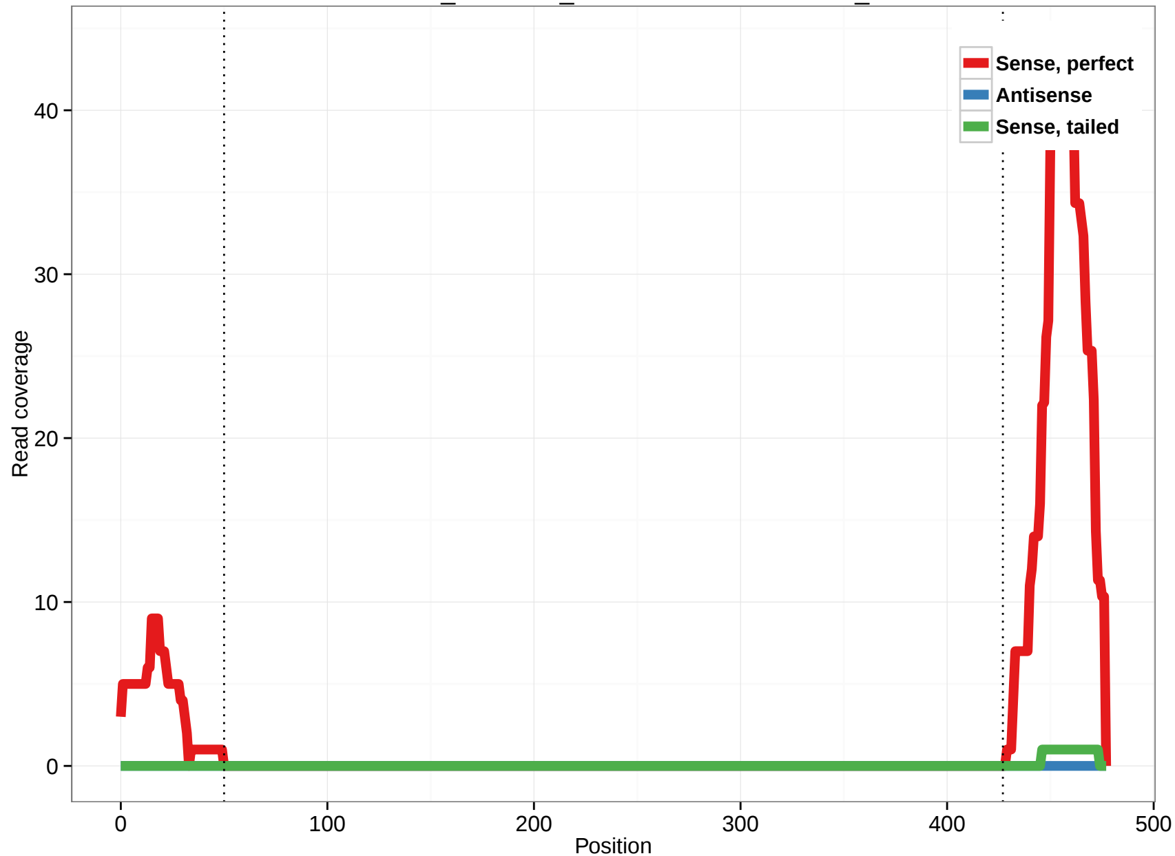
ornAna1_ensGene_ENSOANT00000002926_8
