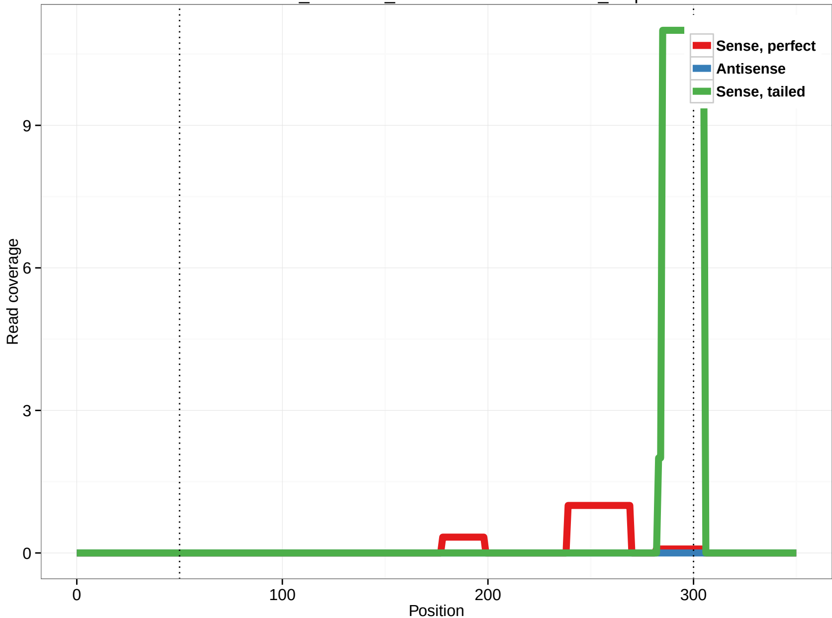
ornAna1_ensGene_ENSOANT00000002847_8.5p
