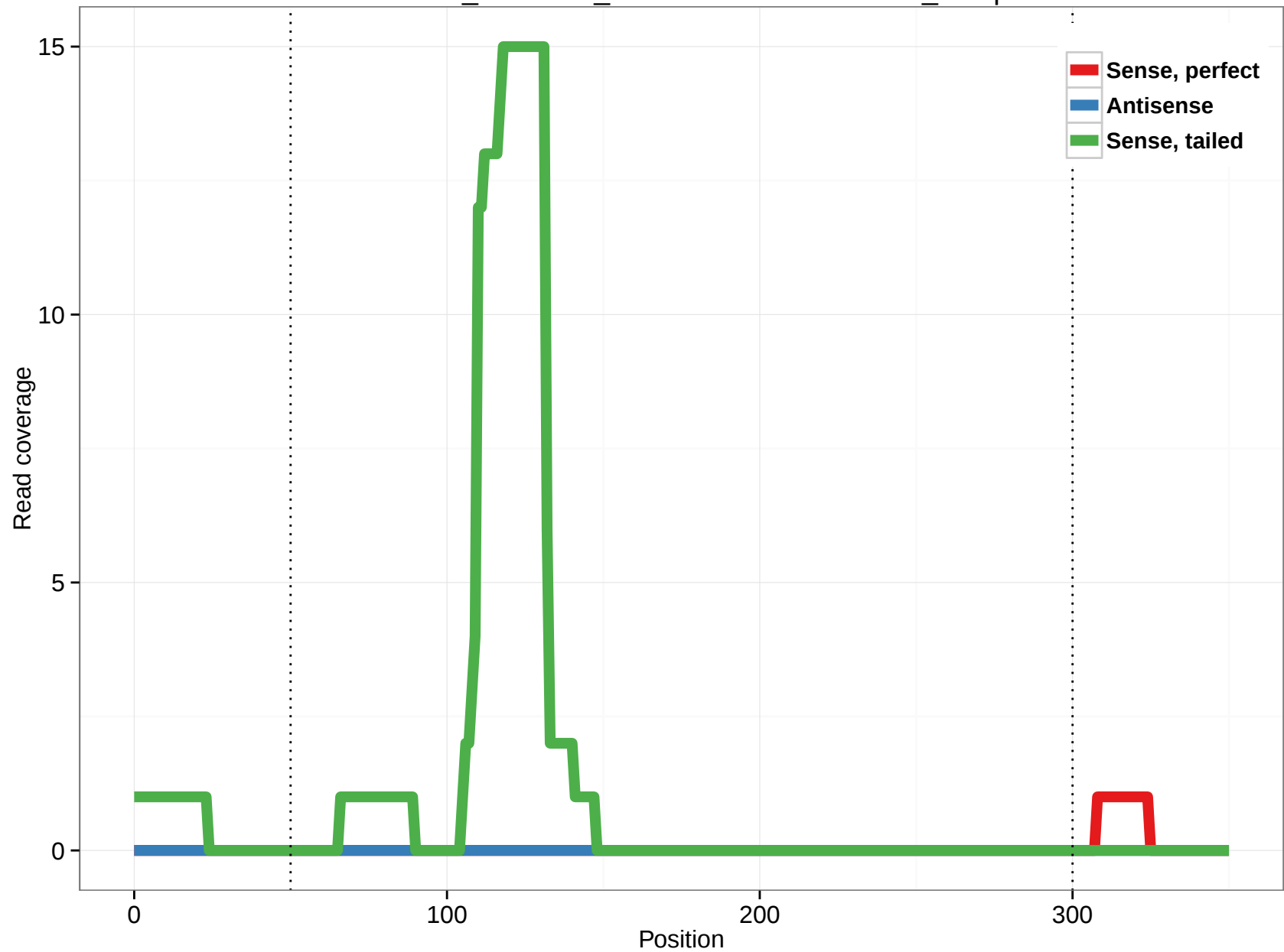
ornAna1_ensGene_ENSOANT00000002824_25.3p
